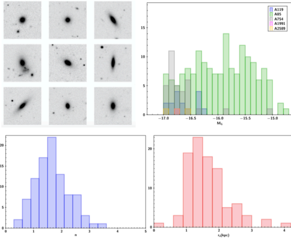
Figure 1. Upper Left panel: A selection of dwarfs FOV 1.6'x1.6' North at top Est at left. Upper Right panel: The distribution of the absolute magnitude M_g for our sample. Lower Left Panel: Distribution of Sersic index. Lower right panel: distribution of R_e .
