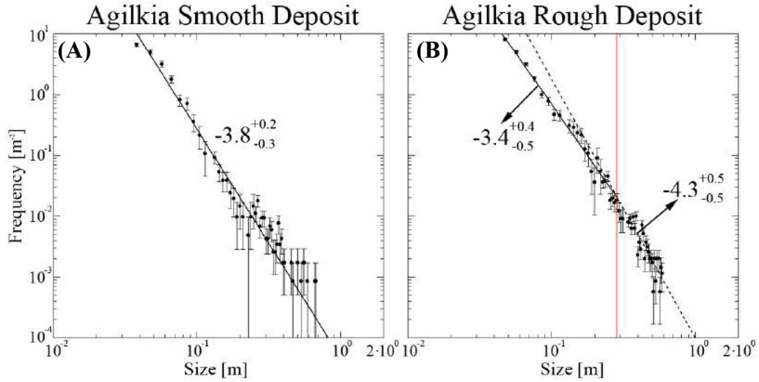
Figure 8. The pebbles/boulders differential SFDs per \text{m}^2 identified on the two units present on Agilkia, i.e. the so-called Smooth (A) and Rough deposits (B). The vertical red line in B indicates the knee of the distribution present on the rough deposit. We here underline that the data used are those of Mottola et al. (2015) but with linear bins. (For interpretation of the references to colour in this figure legend, the reader is referred to the web version of this article.)
