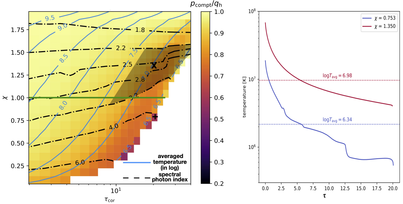
Fig. 3. Left: same map as in Fig. 2 but with the contours of the logarithm of the vertical average coronal temperature (in Kelvin, blue solid line) and the contours of the photon indices of the output spectrum produced by the corona (black dot-dashed lines). The other parameters are fixed to T_{\text{bb}} = 10^5 K, \xi_0 = 10^3 erg s ^{-1} cm, and n_{\text{H}} = 10^{12} cm ^{-3} . Similarly to Fig. 2 the green line corresponds to the condition \chi = 1 . The darkened area corresponds to the usual observational constraints of the temperature (0.1–2 keV) and photon index (2.2–3.2) of the soft X-ray excess. Right: vertical coronal temperature profiles for \tau_{\text{cor}} = 20 and \chi = 1.35 and 0.753 . The corresponding average temperatures T_{\text{avg}} = \frac{1}{\tau_{\text{cor}}} \int_0^{\tau_{\text{cor}}} T(\tau) d\tau are indicated for each temperature profile.
