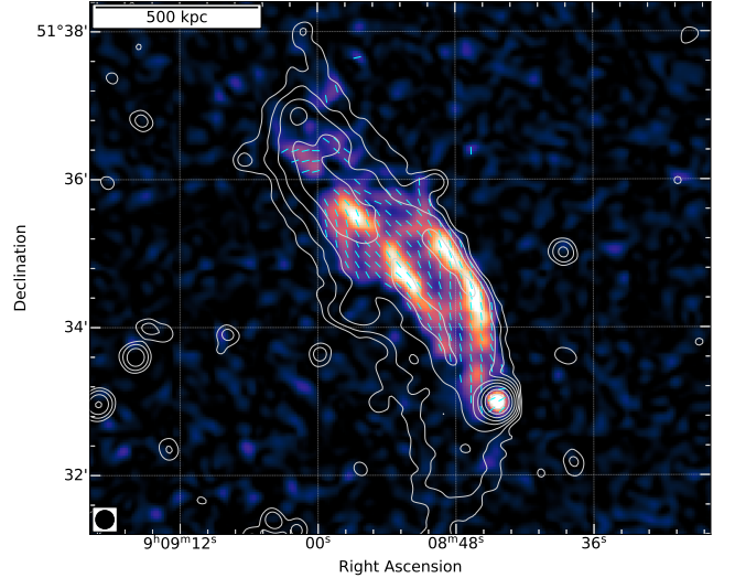
Figure 12. Vector map of the NW relic (at 15'' resolution) showing the orientation of the magnetic field vectors overlaid on the linear polarized intensity image. The vectors are corrected for the Faraday rotation due to the Galactic foreground. The Stokes I contours are from the GMRT 15'' uv-tapered image and are plotted at levels of [1, 2, 4, 8, \dots] \times 4.0\sigma_{\text{rms}} where \text{rms} = 12\mu\text{Jybeam}^{-1} .
