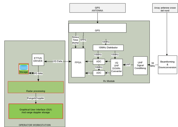
Fig. 4. Receiver architecture
