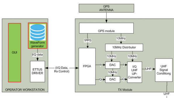
Fig. 3. Transmitter architecture
