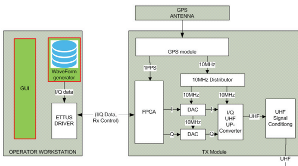
Fig. 3. Transmitter architecture
