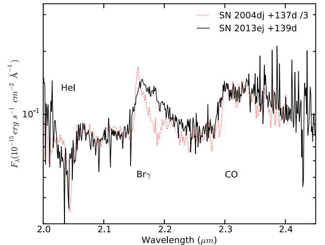
Figure 18. Detection of CO first overtone at day 139, compared to observation at a similar epoch for SN 2004dj (Kotak et al. 2005). Observed flux density of SN 2004dj is reduced by a factor of 3 to be comparable to SN 2013ej.
