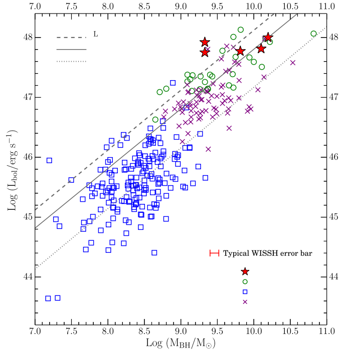
Fig. 4. Bolometric luminosity as a function of the \text{H}\beta -based SMBH mass ( M_{\text{BH}}^{\text{H}\beta} ) for different AGN samples. The WISSH quasars are indicated by red stars, while squares refer to X-ray selected Type 1 AGN from Lusso et al. (2012). Circles and crosses indicate the optically selected z \sim 2\text{--}3 quasars from Shemmer et al. (2004) and Shen (2016), respectively. The lines correspond to L_{\text{Bol}}/L_{\text{Edd}} = 1 (dashed), L_{\text{Bol}}/L_{\text{Edd}} = 0.5 (solid), and L_{\text{Bol}}/L_{\text{Edd}} = 0.1 (dotted).
