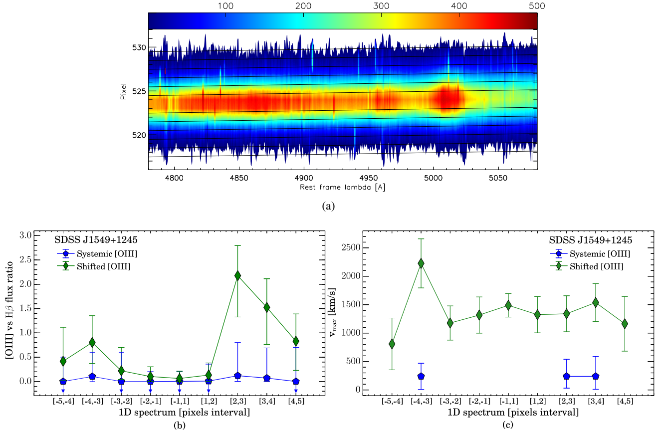
Fig. A.4. Same as Fig. A.1 but for J1549+1245 (1 pixel \sim 2.1 kpc at the redshift of this source).
