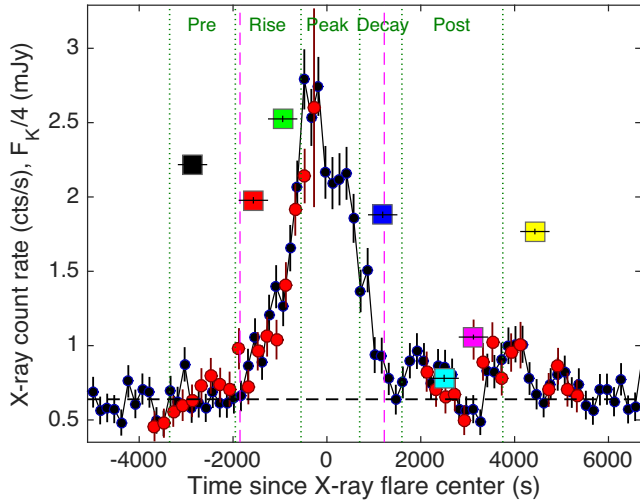
Figure 5. The black and red points show the XMM–Newton 2–10 keV (sum of the three EPIC cameras) and NuSTAR 3–20 keV light curve of Sgr A* flare VB3 (Ponti et al. 2015c), respectively. A constant rate of 0.13 cts s −1 has been subtracted from the NuSTAR light curve for display purposes, to take into account the different contribution of the diffuse and quiescent emission (gaps in the NuSTAR light curve are due to Earth occultation). The squares show the extinction corrected SINFONI light curve of Sgr A* during the VB3 flare. Each point corresponds to an NIR spectrum integration time of 600 s. The y-axis reports the observed renormalized (divided by 4 for display purposes) flux density at 2.2 μm in mJy units. The black dashed line indicates the level of the ‘non-flare’ (quiescent in X-rays) emission. The pink dashed lines indicate the start and end of the XMM–Newton VB3 flare, as indicated by the Bayesian block decomposition (see Ponti et al. 2015c). Excess X-ray emission is observed ~2000 and ~4000 s after the X-ray flare peak. The dotted green lines show the intervals for the integration of the pre-, rise, peak, decrease and post-flare spectra during VB3. The zero-point of the abscissa corresponds to 525831144.7 s (TT TBD ) and 2456900.50784 d (BJD TBD ), respectively.
