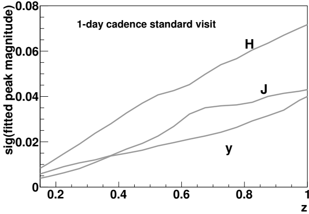
Fig. C.1. Precisions of the fitted amplitude of light curves with a one-day cadence of standard visits, as a function of redshift. The requirement of 0.04 is met at z < \sim 1 in y and J , and z < 0.5 in H .
