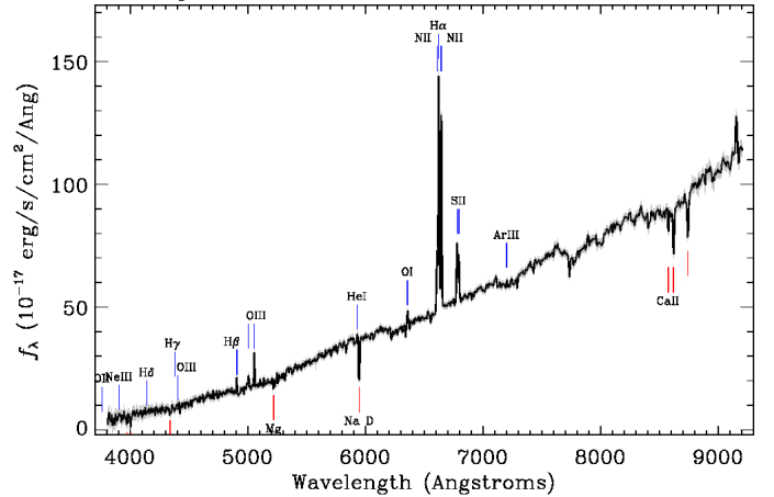
Fig. 1. SDSS spectrum of NGC 2785. The source is characterized by a very red continuum and a large H\alpha/H\beta line ratio (even after correction for the host galaxy contribution), suggestive of a heavily extinguished object (see text and V11 for details). The main emission/absorption lines (as reported in the SDSS webpage) are labeled.
