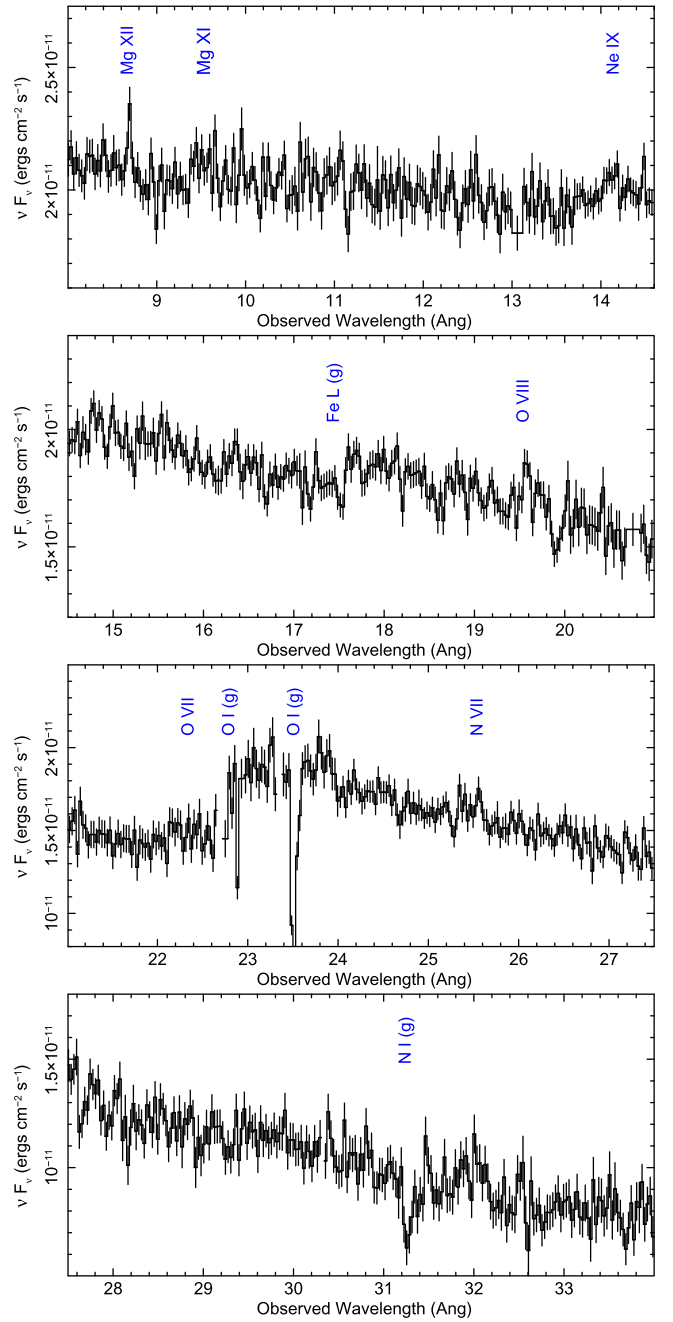
Figure 2. The four panels show the fluxed 2014 RGS spectrum of Ark 120, obtained from combining all four sequences and from the RGS 1 and RGS 2 data. The spectra have been fluxed against a power-law continuum of photon index \Gamma = 2 to create a \nu F_\nu plot and are plotted against wavelength (in Angstroms) in the observed frame. The wavelengths of some of the expected emission lines from abundant elements are indicated, while the predicted position of absorption due to the ISM of our own Galaxy are also marked (denoted with a g symbol). Note the strong absorption lines and edge due to neutral O and N from our own Galaxy, as well as the possible presence due to photoionized emission lines from N, O, Ne, and Mg in the restframe of Ark 120.
