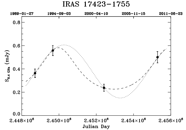
Figure 2. VLA observations at 8.4 GHz of IRAS 17423-1755 over 16 years. The point in 1991 is from the VLA project AK247 (PI: Knapp), while that from 1993 is from AZ63 (PI: Zijlstra).
