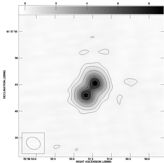
Figure 5. Bipolar morphology observed at 8.4 GHz in IRAS 22568+6141. The contours are 60 \times (-3, 3, 9, 27, 81, 100, 130) \mu\text{Jy}/\text{beam} and the grey scale is in \text{mJy}/\text{beam} . The convolution beam is shown in the bottom left corner.
