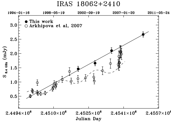
Figure 4. Radio flux density at 8.4 GHz and H_\beta flux (Arkhipova et al 2007) at several epochs for IRAS 18062+2410. The dashed curve is a fit to the H_\beta points before 2002.
