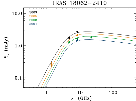
Figure 3. Radio continuum spectra of IRAS 18062+2410 obtained at different epochs. The correspondent model curves are shown in the same colour as the data points.
