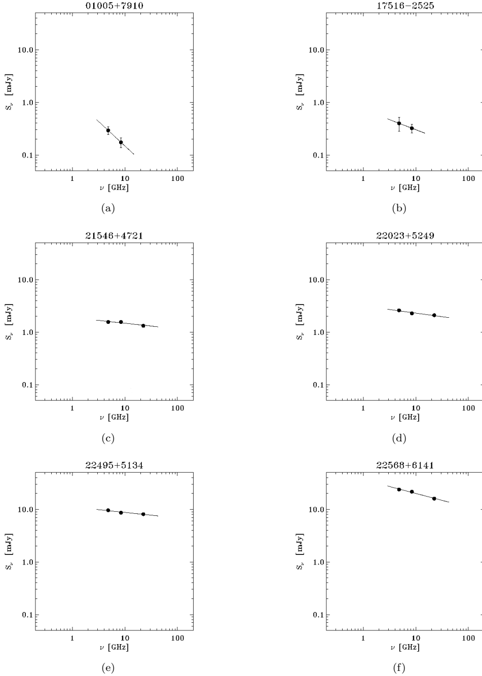
Figure 1. Continuum spectra for targets that had not been observed before at radio wavelengths or that lacked multi-frequency observations.
