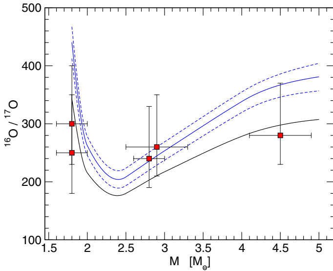
Fig. 4. ^{16}\text{O}/^{17}\text{O} ratios after the first dredge-up versus stellar mass in M_\odot . Lines represent the theoretical predictions, and the red squares are observations. Blue solid line: reference model (R). Blue dashed lines: ^{17}\text{O} proton capture rate modified within the suggested upper and lower rates (O17L and O17H). Solid black line: theoretical predictions as obtained by reducing the initial ^{16}\text{O} to [\text{O}/\text{H}] = -0.22 (C16OL).
