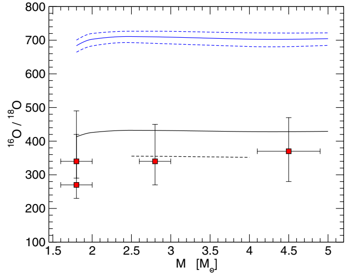
Fig. 5. ^{16}\text{O}/^{18}\text{O} ratios after the first dredge-up versus stellar mass in M_\odot . Lines represent the theoretical predictions, and the red squares are observations. Solid blue line: reference model (R). Dashed blue lines: ^{18}\text{O} proton capture rate modified within the suggested upper and lower rates (O18L and O18H). Solid black line: model predictions obtained by reducing the initial ^{16}\text{O} to [\text{O}/\text{H}] = -0.22 (C16OL). Dashed black line: model with the initial ^{18}\text{O} abundance increased by a factor of 2 (C18OHH).
