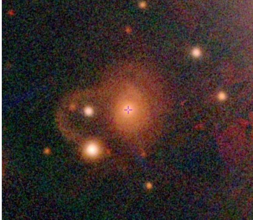
Figure 29: Optical image of source #4 from Pan-STARRS.
