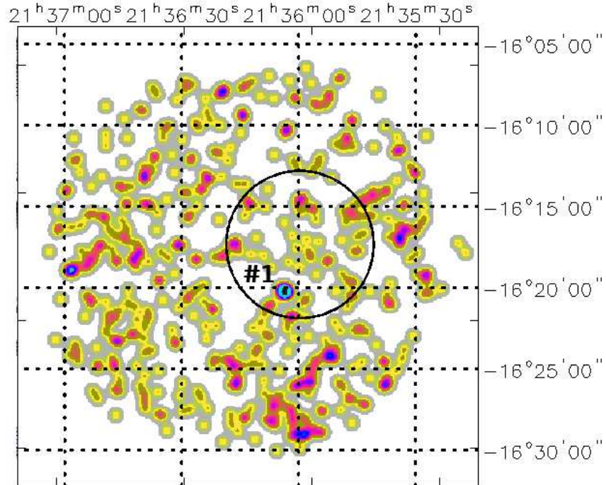
Figure 47: 0.3–10 keV XRT image of the PBC_NEW_330 field.
