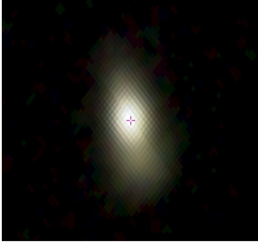
Figure 6: Optical image of source #1 from SDSS.
