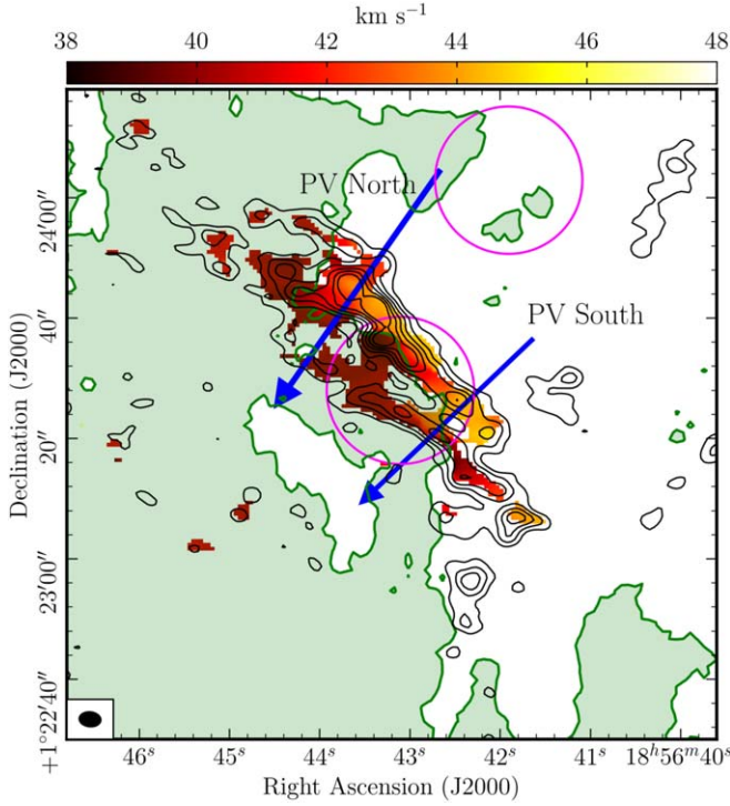
Figure 2. SiO integrated intensity map (black contours; velocity range 36.6–47.6 km s −1 ) toward G034 superimposed on its moment 1 velocity map (red scale). Contours are from 3σ (σ = 0.016 Jy km s −1 ) by steps of 3σ. Green contour and shadow indicates the A v ≥ 20 mag dense material in the IRDC (Kainulainen & Tan 2013). Blue arrows show the directions used to extract the PV diagrams of Figure 4. Magenta circles indicate the two positions used to estimate the gas density conditions. Beam size is indicated as a black ellipse in the bottom left corner.
