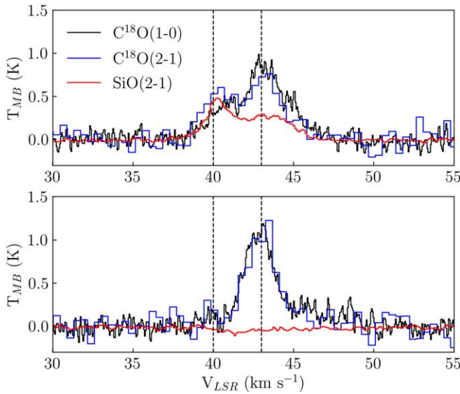
Figure 5. Spectra of \text{C}^{18}\text{O}(1-0) (black lines), \text{C}^{18}\text{O}(2-1) (blue lines), and \text{SiO}(2-1) (red lines) extracted toward G034 at positions \alpha(\text{J2000}) = 18^{\text{h}}56^{\text{m}}43.1^{\text{s}} , \delta(\text{J2000}) = 1^{\circ}23'28'' (top panel) and \alpha(\text{J2000}) = 18^{\text{h}}56^{\text{m}}41.9^{\text{s}} , \delta(\text{J2000}) = 1^{\circ}24'03'' over a 25'' beam. The components at 43^{\circ} and 40^{\circ} \text{km s}^{-1} corresponds to pre-shock and post-shock gas, respectively (vertical dashed lines).
