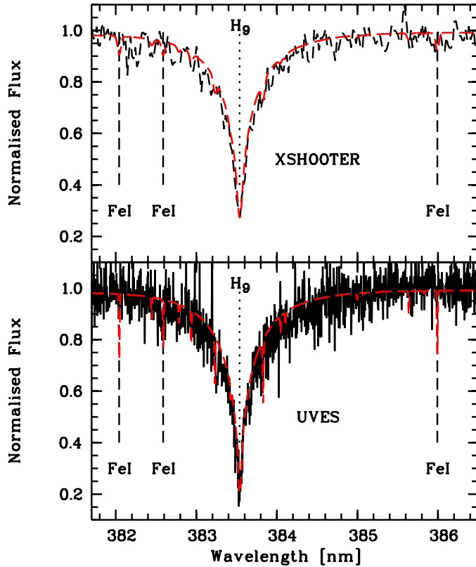
Fig. 4. SDSS J1035+0641: the X-Shooter (top panel) and UVES (bottom panel) spectra in the region covering the three strongest Fe I lines. The comparison spectrum is a synthetic spectrum computed with [\text{Fe}/\text{H}] = -4.5 .
