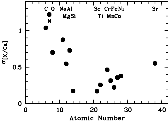
Fig. 8. \sigma [X/Ca] for elements that are measured in at least two of the nine CEMP stars (HE 0107-5240 HE 1327-2326, HE 0557-4840, HE 0134-1519, HE 0233-0343, HE 1310-0536, SMSS J0313-6708, CS 22949-037, and G 77-61), as a function of atomic number. As in Fig. 7, C and N in CS 22949-037 were not taken into account.
