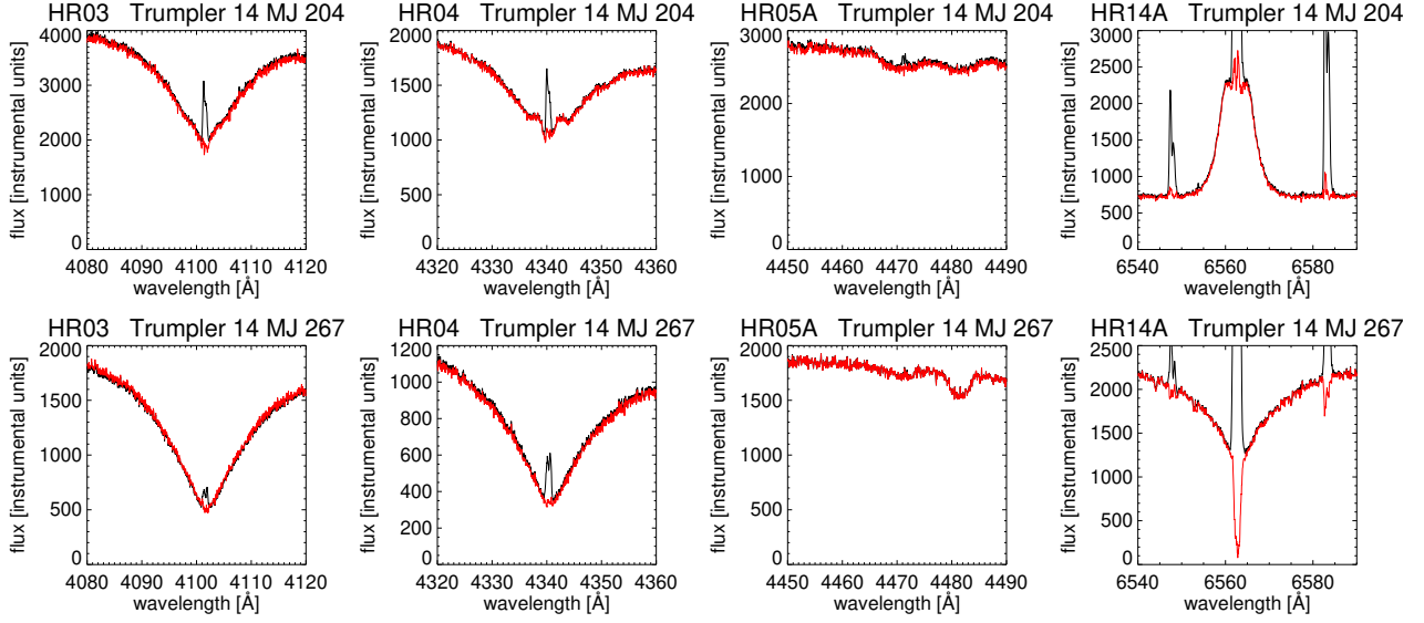
Fig. 2. Two examples of the nebular correction that has been applied to stars in the Carina Nebula. The black line shows the original spectrum, the red line the corrected spectrum. The effect is largest for H \alpha and the [N II] lines (HR14A setup) and becomes smaller for H \gamma (HR04) and H \delta (HR03). The effect on He I \lambda 4471.5 (HR05A) is very small.
