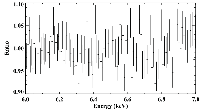
Figure 4. The 6.0–7.0 keV data/model ratio fit using the DISKLINE model. The data are unbinned with bin sizes of \sim 0.008 keV. It can be seen that no obvious emission or absorption features presenting in the figure.
