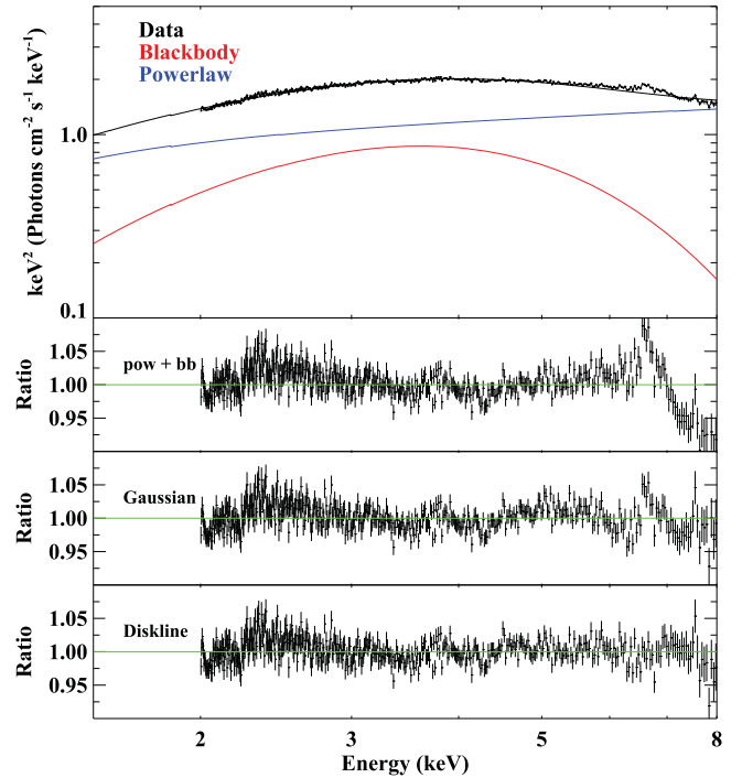
Figure 2. Top panel: the unfolded spectrum of Serpens X-1 with decomposed model components. We display the data/model ratios of the continuum model tbabs*(bbbody + power-law) Model 3, and Model 3a in the lower panels.
