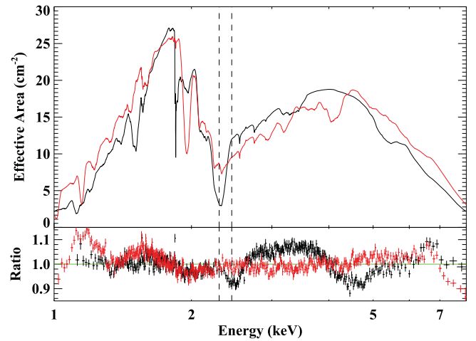
Figure 6. HEG +1 (in black) and –1 (in red) detector effective areas in the upper panel. The lower panel of the figure shows the Serpens X-1 HEG +1 (black data points) and –1 (red data points) data/model ratios. The continuum is modeled as \text{tbabs}*(\text{diskbb} + \text{bbody} + \text{power-law}) . The plot reveals the poor calibration of the HEG +1 spectrum. The vertical dashed lines are intended to help guide the eye.
