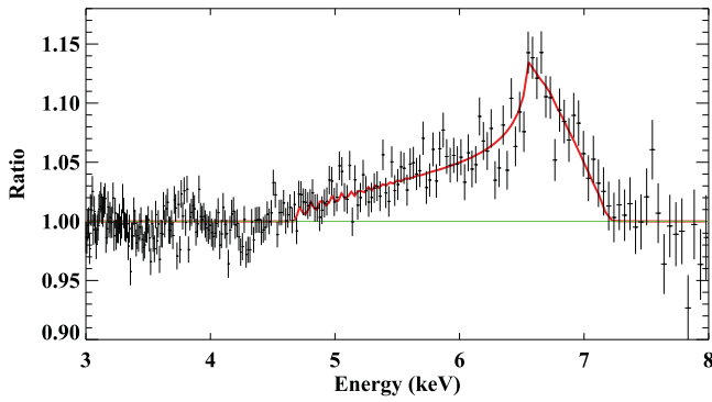
Figure 3. Fe line profile of Serpens X-1. The spectrum is modeled as tbabs (bbody + power-law + diskline) , and the plot is produced by setting the normalization of DISKLINE to be 0. The plot is visually binned with “seplot rebin” in XSPEC. The bin sizes through the Fe line are \sim 0.042 keV. The red line shows model. It can be seen that the DISKLINE model fits the asymmetric line very well.
