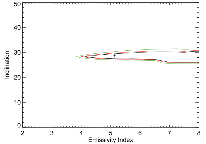
Figure 5. Contour plot of the emissivity index against the inclination angle, which was calculated from the REFLIONX model. The contours are plotted at 67% (black), 90% (red), and 99% (green) confidence levels. It can be seen that there is no clear degeneracy between emissivity and inclination angle.
