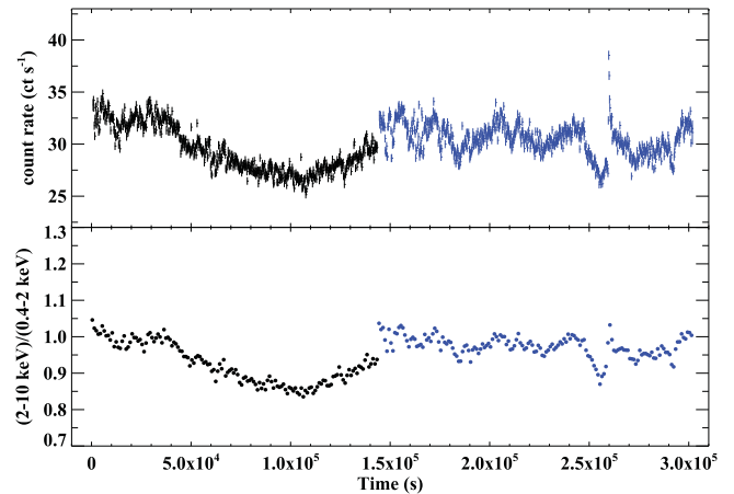
Figure 1. Upper panel: the 0.4–10 keV light curve of Serpens X-1. The light curve was extracted from the first-order HEG data. The gap between the observations has been discarded. Black points stand for data extracted from the first half of the observation, and blue ones for the second. There is a weak type I X-ray burst containing \sim 0.5\% of the total counts in the second half of the observation. Lower panel: the hardness ratio, which is the hard (2–10 keV) light curve divided by the soft (0.4–2.0 keV) light curve.
