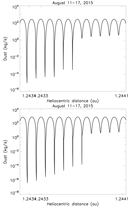
Figure 6. Case 1 (upper panel) and Case 2 (lower panel), location A, 2015 August 11–17: dust flux.
