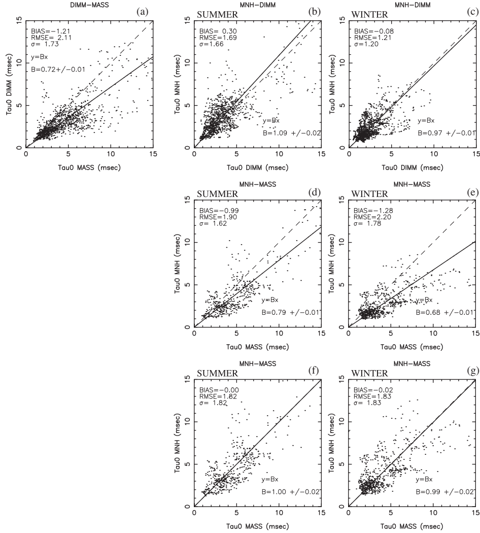
Figure 5. Scattered plots (validation sample) of the wavefront coherence time \tau_0 between (a) MASS and DIMM – 48 nights in 2010/2011 (there are no MASS measurements in 2007); (b) MESO-NH and DIMM in summer – 42 nights in 2010/2011; (c) MESO-NH and DIMM in winter – 47 nights in 2010/2011; (d) MESO-NH and MASS in summer – 21 nights in 2010/2011; (e) MESO-NH and MASS in winter – 27 nights in 2010/2011; (f) the same as (d) but with the MASS corrected using the coefficient of the regression line from (d); and (g) the same as (e) but with the MASS corrected using the coefficient of the regression line from (e). For the model performances, the key panels to take into account are (b), (c), (f) and (g). See extended discussion in the text.
