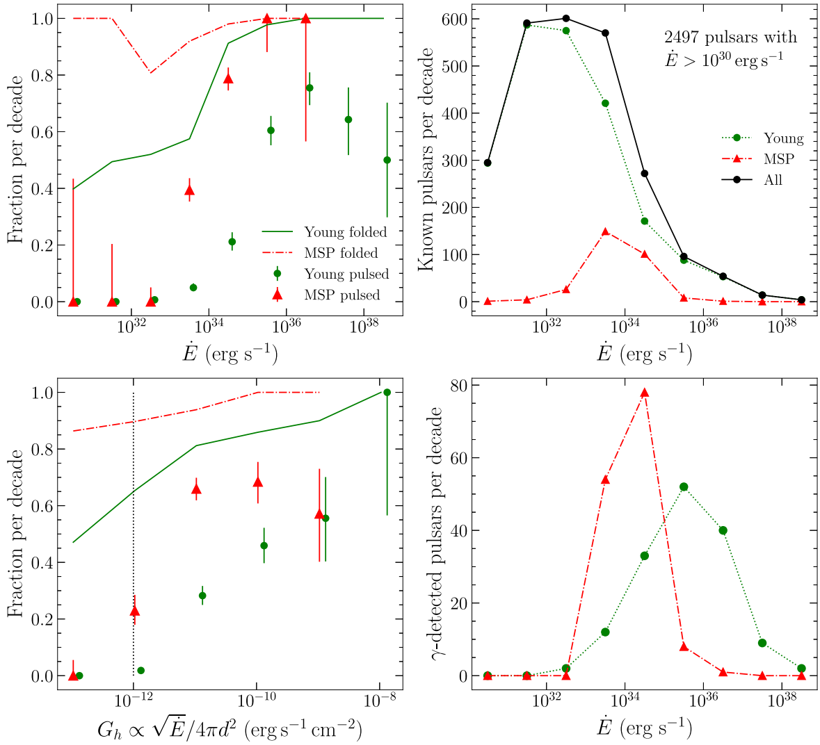
Figure 5. Left-hand plots: the lines show the fractions of known field pulsars that have been gamma-folded, vs. spin-down power \dot{E} (top) and, when a distance estimate exists, the heuristic gamma-ray flux G_h defined in Section 7.1 (bottom). The points show the fractions of folded pulsars for which pulsations have been detected. The vertical dotted line approximates the minimum detectable integral energy flux G_{100} . Right-hand plots: numbers of known and gamma-ray detected field pulsars vs. \dot{E} . (A quarter of ATNF psrcat pulsars have unmeasured \dot{E} .) An earlier version of this figure appears in Laffon et al. (2015).
