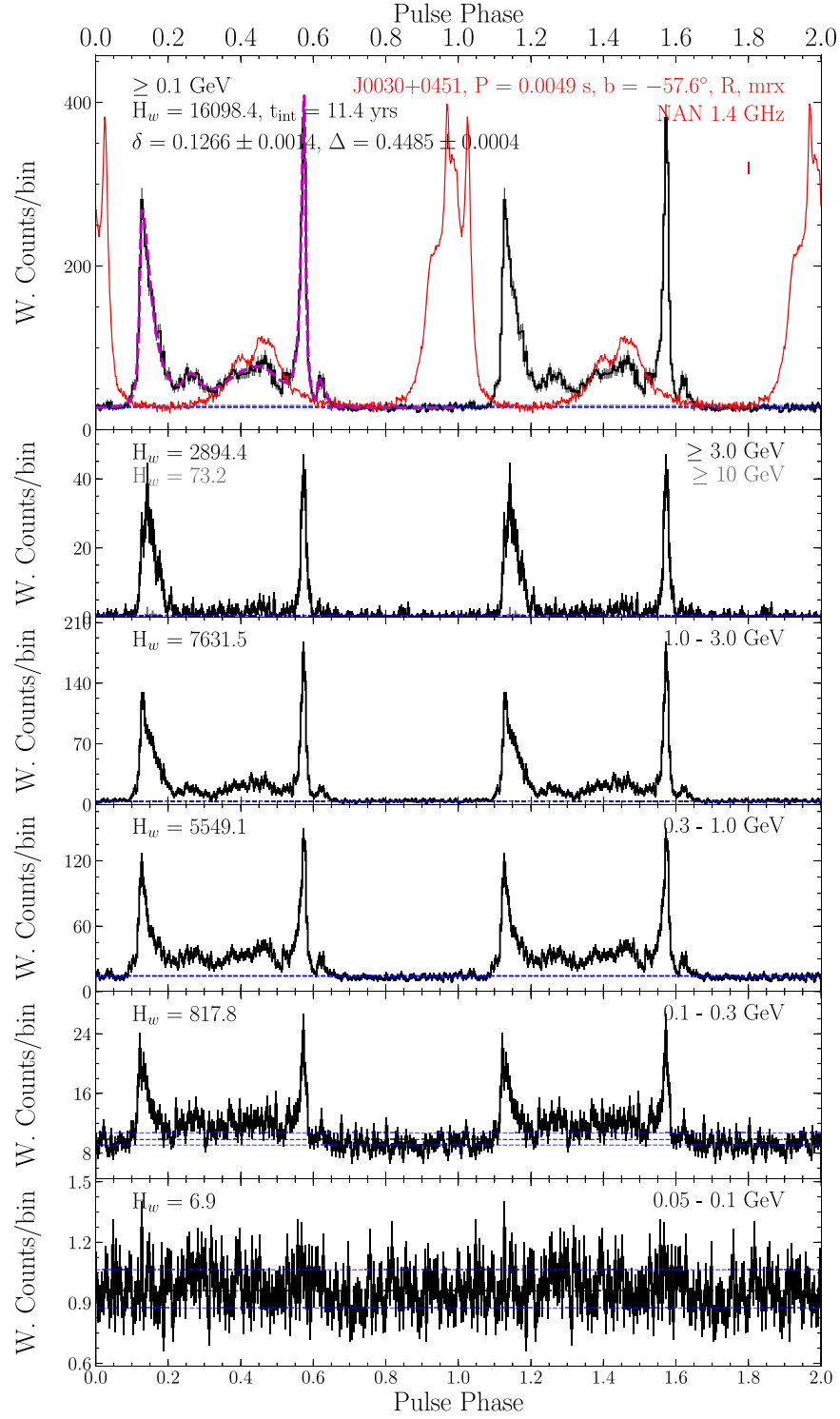
Figure 9. Pulse profiles for the MSP PSR J0030+0451. Weighted LAT pulse profiles in different energy bands are shown in black. The pulse profiles above 10 GeV are in light gray, more apparent for other pulsars shown in Appendix B. The radio pulse profile for this pulsar at 1.4 GHz is shown in red, and a fit of the integrated gamma-ray pulse profile over 0.1 GeV is displayed in magenta when the H -test test significance exceeds 100. Horizontal blue lines correspond to the expected background levels in the gamma-ray pulse profiles, plus or minus one standard deviation. The quantities at the top left correspond to the weighted H -test TS for the LAT pulse profile shown in the top panel, and the total integration time. At top right are listed: the pulsar name, its rotational period and Galactic latitude, and the “PSR” and “CHAR” codes defined in the captions for Tables 2 and 3 (top row), the radio observatory used to acquire the radio profile (if available), and the corresponding radio frequency (second row). For pulsars with radio profiles, a marker at the top right indicates the phase alignment uncertainty stemming from the DM. See Section 5 for more details about light-curve construction and the fitting procedure.
