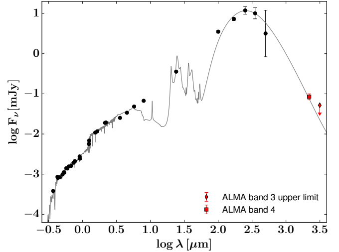
Fig. 2. Multi-wavelength spectral energy distribution of 3D-HST GS30274. The best fit from the MAGPHYS analysis is plotted as a line. The optical, NIR, Herschel measurements are shown as bold circles. The ALMA band 4 continuum detection is presented as a red square. The red diamond represents the three sigma upper limit on the ALMA band 3 continuum.
