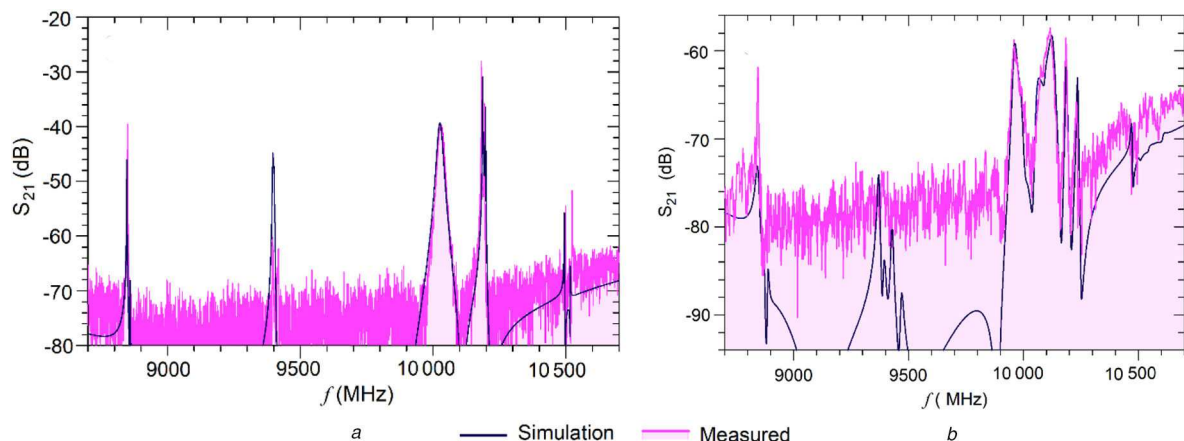
Fig. 10 Simulated and measured responses near the 3rd harmonic
