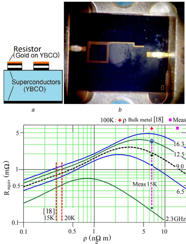
Fig. 2 Equivalent sheet resistance of a combined gold/YBCO bilayer, 200 and 600 nm thick
