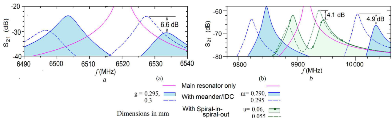
Fig. 4 Frequency staggering and attenuation from the parasitic resonators. Fixed dimensions are given in Fig. 3
