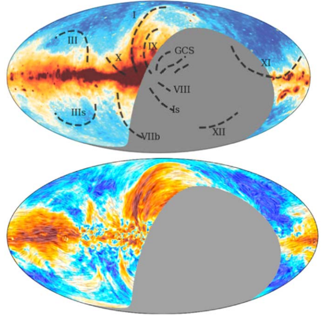
Figure 5. C-BASS North maps of total intensity (top) and polarized intensity (bottom) in Galactic coordinates using a Mollweide projection. The total intensity map color scale has been saturated along the Galactic plane and includes the locations of well-known radio loops (Vidal et al. 2015). The polarized intensity map has the projected B-field direction overlaid using line-integral convolution.
