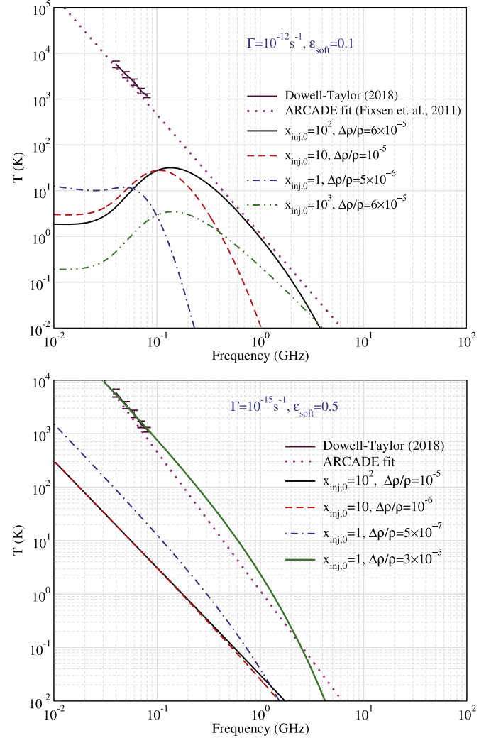
Figure 8. Spectral distortion signals created by free-free-type soft photon injection from a decaying dark matter particle with lifetime t_x \simeq 10^{12} s (top) and 10^{15} s (bottom). In each case, it is assumed that a fraction \epsilon_{\text{soft}} of the total energy (as labeled) is injected as soft photons. The injection frequency, x_{\text{inj},0} = h\nu_{\text{inj},0}/kT_0 , is also varied with some of the cases shown coming intriguingly close to the ARCADE RSB level (figures provided by Sandeep Acharya).
