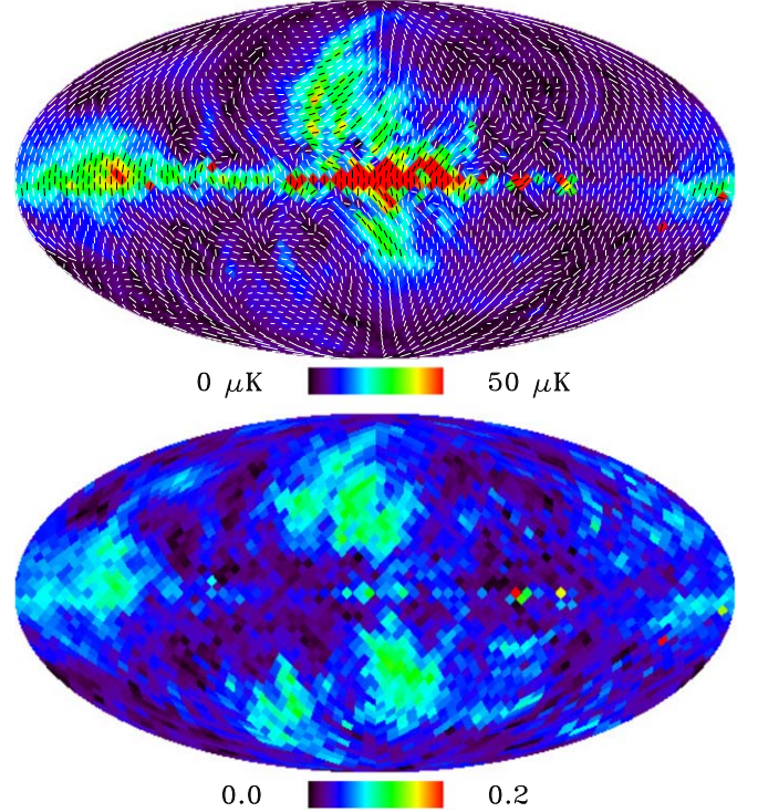
Figure 14. Polarization intensity P (top) and fractional polarization P/I (bottom) from Planck evaluated at 30 GHz. Despite the high degree of depolarization, the polarization angle (white bars) shows little scatter.
