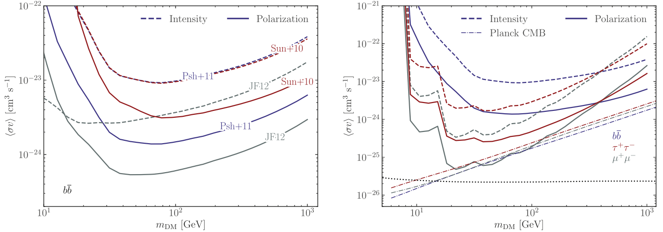
Figure 19. Upper limits on the DM annihilation cross section from the intensity and polarization data at 30 GHz. Left: effect of the GMF modeling for the \bar{b}b channel. Right: constraints for different annihilation channels for the Psh+11 GMF. Also shown for comparison are the constraints obtained from Planck CMB data (Aghanim et al. 2020b).
