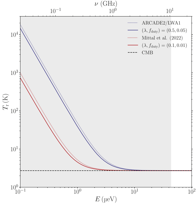
Figure 12. The net background temperature ( T_r = T_b + T_{\text{CMB}} ) generated by radio emission due to accretion onto supermassive PBHs. For \lambda = 0.5 , f_X = 0.1 , f_{\text{duty}} = 0.05 , and f_{\text{PBH}} = 10^{-4} (solid blue), we can explain the RSB observed (dotted blue). For \lambda = 0.1 , f_{\text{duty}} = 0.01 we get (solid red) 5% of ARCADE 2 (dotted red) radio emission necessary to get the EDGES result (Mittal et al. 2022). The CMB temperature is shown in dashed black for reference. The gray shaded region roughly covers the frequency range over which an RSB has been seen.
