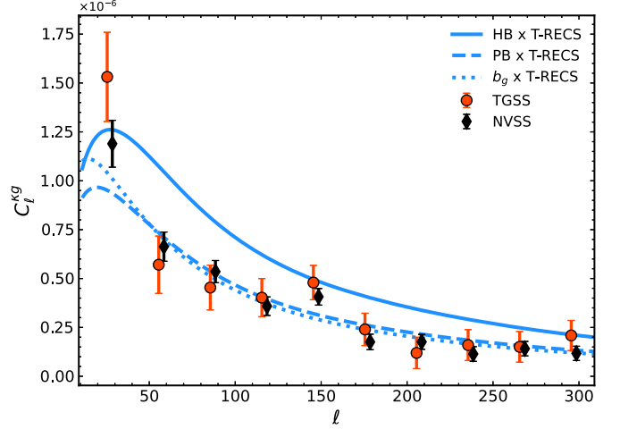
Figure 7. Measured cross-spectrum \kappa g of TGSS–CMB lensing (red dots) and NVSS–CMB lensing (black diamonds). Error bars represent the 1\sigma uncertainties obtained assuming Gaussian statistics. Blue curves represent model predictions obtained using different prescriptions for the bias, b(z) , while the T-RECS N(z) distribution of Bonaldi et al. (2018) is used (see Piccirilli et al. 2022 for a detailed description).
