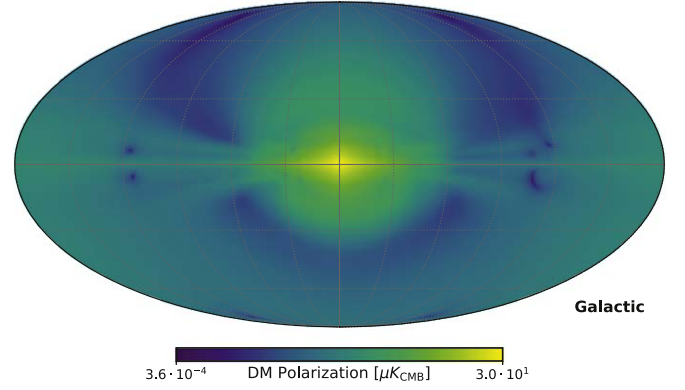
Figure 18. Example morphology of the DM synchrotron Polarization amplitude at 30 GHz for m_{\text{DM}} = 50 GeV annihilating in \mu^+\mu^- pairs with a thermal cross section and the Psh+11 GMF model.
