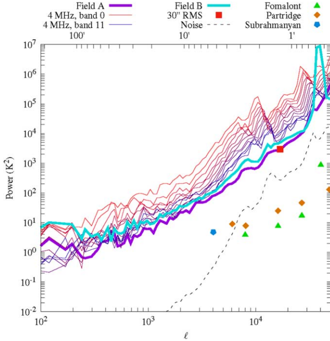
Figure 4. Measured anisotropy power spectrum of the radio sky centered at 140 MHz with an rms noise of 720 \mu Jy. Shown are curves for the full bandwidth of the coldest patch field (field A) and the secondary field (field B), as well as for twelve 4 MHz wide subbands of field A. The anisotropy in field A deduced by considering the average noise per beam in the image with the synthesized beam tapered to 30'' FWHM is also shown and agrees at the relevant angular scale. We also show comparison levels inferred by the noise per beam at 8.7, 8.4, and 4.9 GHz in different fields as calculated by Holder (2014) and scaled here to 140 MHz assuming a synchrotron power law of -2.6 in radiometric temperature units. The amount of angular power is \sim 1.4 times higher for field B compared to field A (in K^2 units) across a range of angular scales. All angular powers are expressed here in the (\Delta T)_\ell^2 normalization. Reproduced from Offringa et al. (2022).
