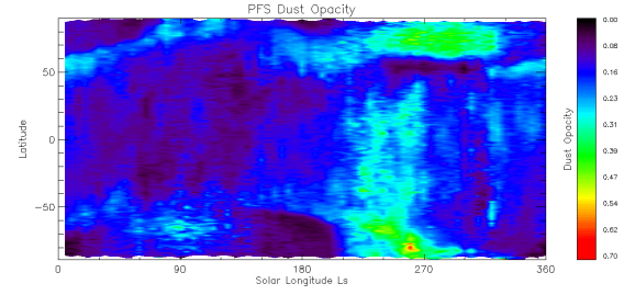
Fig.4 Seasonal evolution of dust opacity
