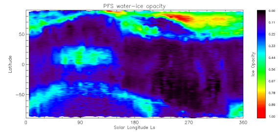
Fig.5 Seasonal evolution of ice opacity
