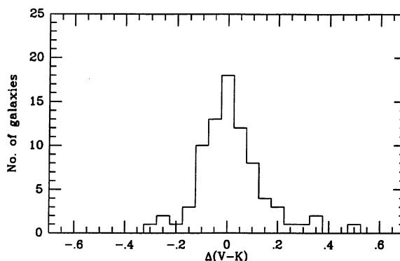
FIG. 14. Same as Fig. 13 but plotted as histogram of the V - K residuals (80 galaxies available). The scatter of the distribution is \sigma = \pm 0.13 mag. See text for discussion.
