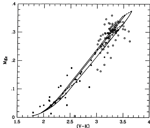
FIG. 11. Adopted calibration for Mg_2 in stellar systems. Upper, central, and lower lines are, respectively, for 15 Gyr SSPs with s = 1.35, 2.35 , and 3.35 . Dashed lines within the strip mark increasing metallicity Z = 0.0001, 0.001, 0.01, 0.017, 0.03 , and 0.1 . Open dots are elliptical galaxies from Davies et al. (1987), while full dots and asterisks are Galactic and M31 globular clusters are from Burstein et al. (1984). See text for details and discussion.
