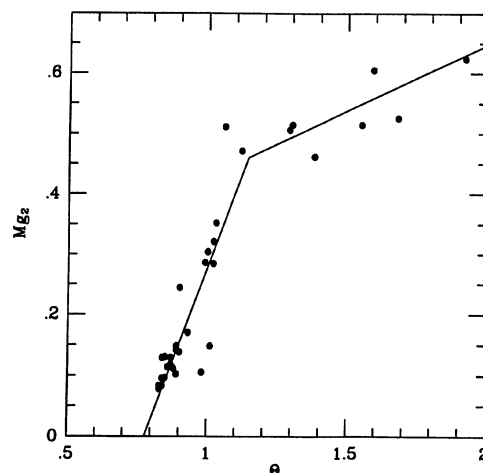
FIG. 6. The effect of the break in the increasing rate of \text{Mg}_2 at low temperatures. Displayed are 33 stars from the working sample with metallicity about solar ( [\text{Fe}/\text{H}] = \pm 0.25 dex) and \log g > 3 . The fitting relation for \log g = 4.0 is also reported.
