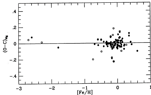
FIG. 8. Same as Fig. 7, but vs [\text{Fe}/\text{H}] . Once more no systematic trends seem to appear.
