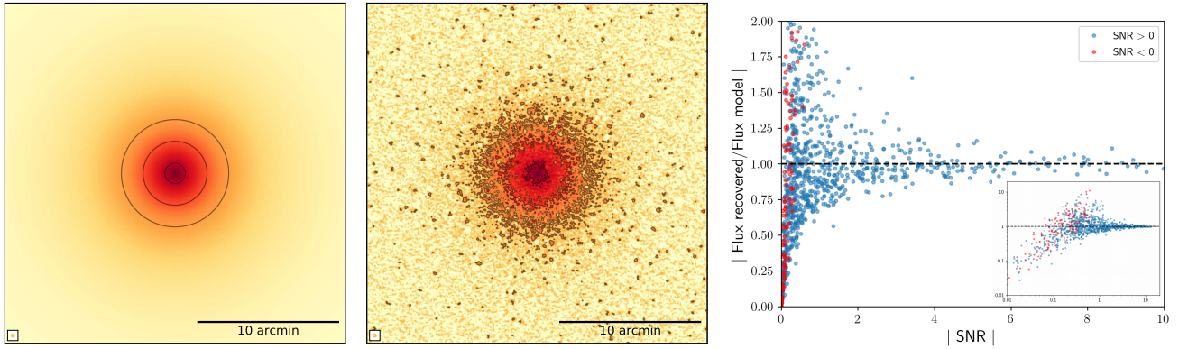
Figure 11. Exponential radio halo model injected in the visibilities ( left ) and corresponding restored image ( center ) at the same resolution of 15'' \times 15'' . The colorscale in the two images is matched and contours/circles are drawn at levels of 120 \times [3, 6, 12] \mu\text{Jy beam}^{-1} . The absolute value of the ratio between recovered flux and injected flux as a function of the absolute value of the SNR ( right ) has been computed on a point-to-point basis from the images shown in the other two panels. The inset shows a zoom-out of the panel plotted in log-scale.
