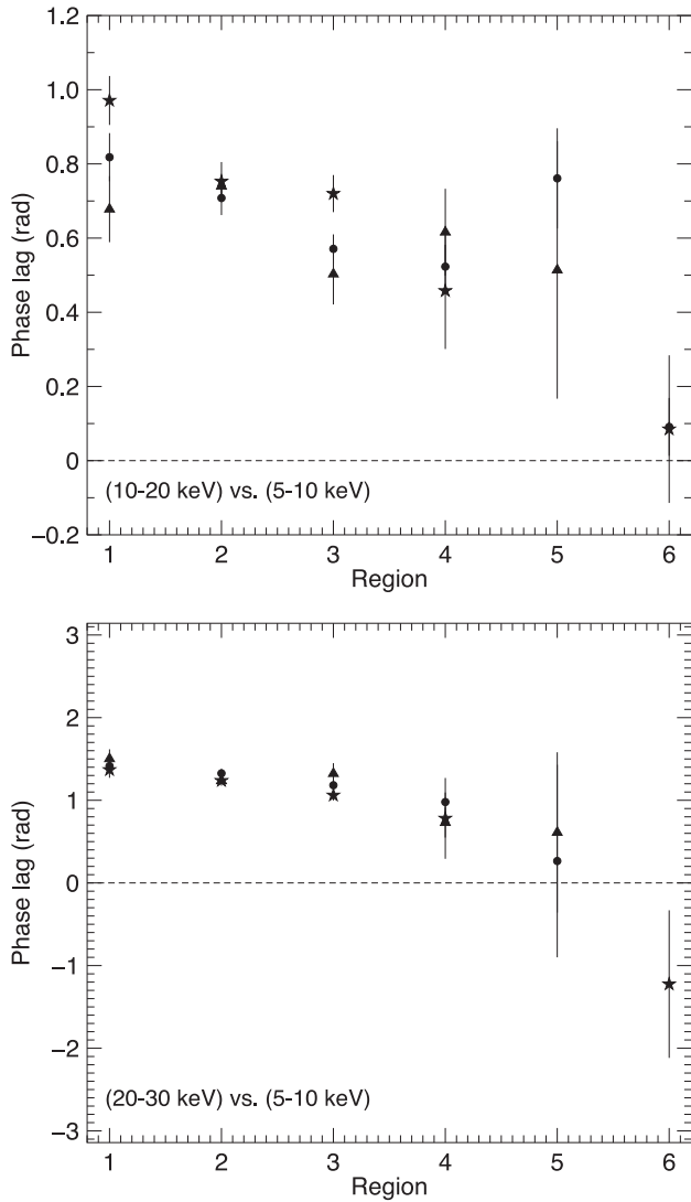
Figure 7. Phase lags at the HFQPO as a function of H I/Ds region for the three selection groups. All frequencies have an error bar, often within the symbol. Top: 10–20 keV versus 5–10 keV. Bottom: 20–30 keV versus 5–10 keV.
