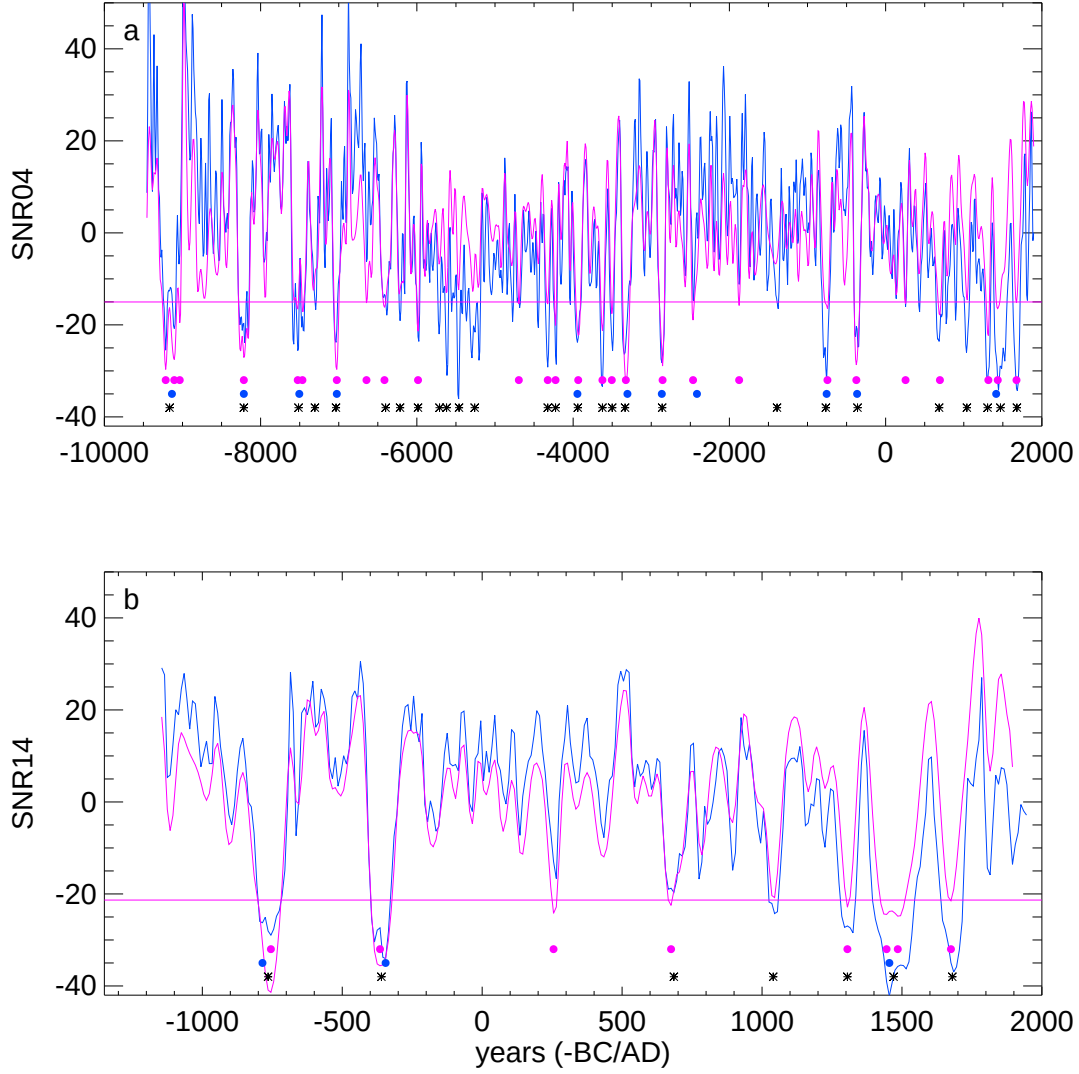
Fig. 9. Sunspot number (blue line) for the two datasets SNR04 (panel a) and SNR14 (panel b) and respective empirical mode decomposition (magenta line) reconstructions through modes j = 1 - 4 (panel a) and j = 1 - 5 (panel b). Horizontal magenta lines indicate the 90th percentile of the EMD reconstruction distribution function. Magenta dots correspond to times when the EMD reconstructions (magenta lines) are beyond the 90th percentile of its distribution function. Blue dots mark the times when the EMD derived Suess cycle is beyond the 90th percentile. Black asterisks correspond to the grand minima identified in Usoskin et al. (2007).
