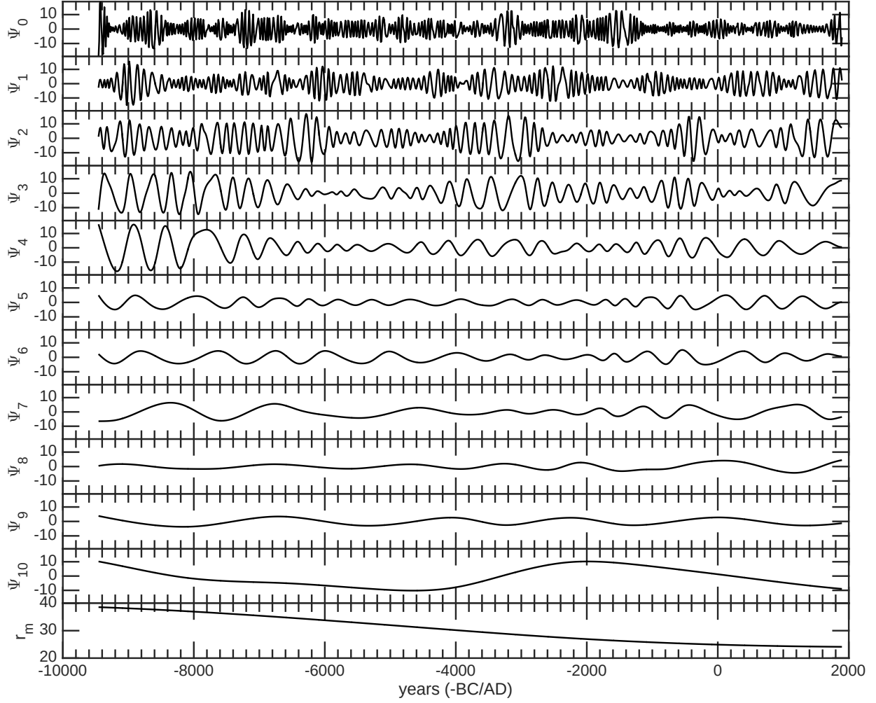
Fig. 5. Empirical mode decomposition modes \psi_j and the residue r_m(t) for the sunspot number SNR04 dataset (Solanki et al. 2004).
