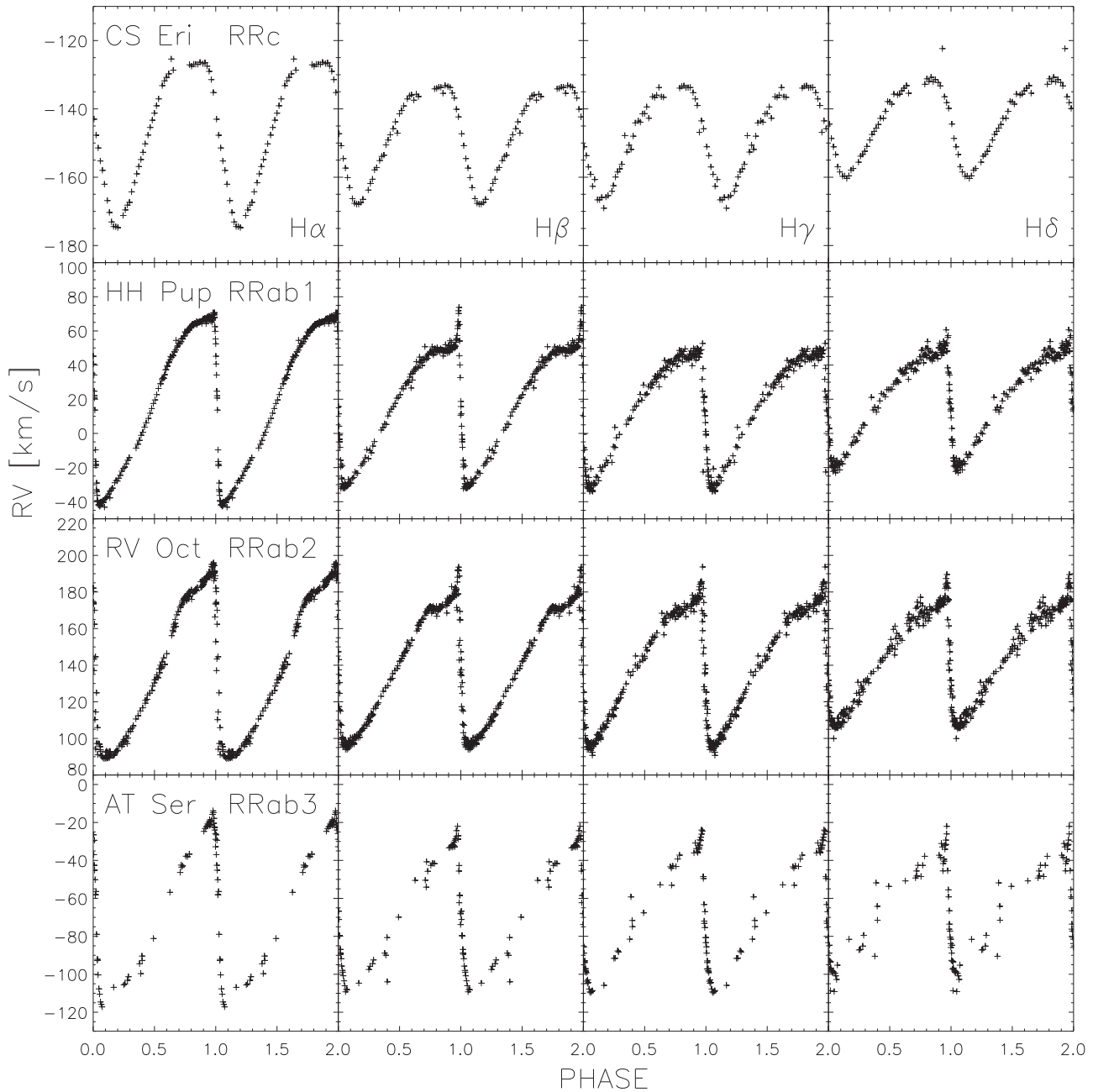
Figure 11. First row: from left to right, radial velocity curves of the RRc variable CS Eri for individual Balmer lines ( H\alpha , H\beta , H\gamma , and H\delta ). Second row: same as the top, but for the R Rab1 variable HH Pup. Third row: same as the top, but for the R Rab2 variable RV Oct. Fourth row: same as the top, but for the R Rab3 variable AT Ser.
