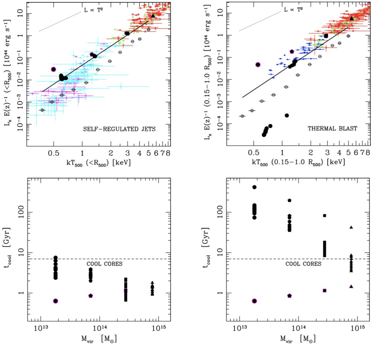
Figure 8. Effects of different baryonic models in shaping the evolution of the hot halos, in particular the X-ray luminosity–temperature relation ( top panels ) and cool-core evolution via the central cooling time ( bottom panels ); adapted from Anderson et al. [103] and Gaspari et al. [27]. The colored individual objects in the top panels are from a wide range of observational works (Helsdon and Ponman [92], Osmond and Ponman [94], Mulchaey et al. [218], Pratt et al. [30], Sun et al. [81], Maughan et al. [219]; luminosities are extracted mostly in the 0.5–2 keV band). The empty circles and solid line show the raw Anderson et al. [103] stacking analysis and the unbiased fit, respectively. The filled black points show evolutionary tracks in large-scale HD simulations (Gaspari et al. [27]) implementing self-regulated AGN jets ( left ) or strong thermal blast feedback ( right ), preserving or evacuating the surrounding diffuse gaseous halo, respectively. The initial state is marked with magenta contour. Evacuation and overheating becomes particularly dramatic in low-mass, less-bound groups.
