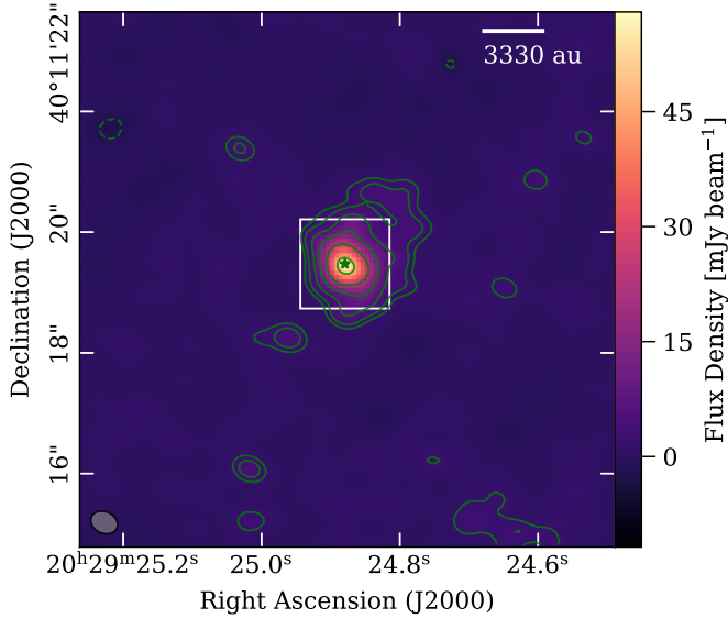
Fig. 2. AFGL 2591 continuum emission at 1.37 mm. The green contours show the 1.37 mm continuum emission with levels at -3 (dashed), 3 , 5 , 10 , 20 , 40 , and 80\sigma ( \sigma = 0.59 \text{ mJy beam}^{-1} ). The beam size ( 0.''46 \times 0.''36 ) is shown in the lower left corner. The green star indicates the position of the 1.37 mm continuum peak. The white rectangle shows the region within which an average spectrum was obtained in the spectral line data for line identification (Sect. 3.2).
