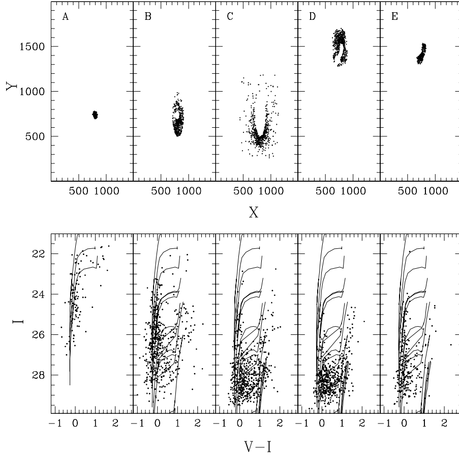
Fig. 1. Upper panels: spatial distribution of the stars in regions A, B, C, D and E in I Zw 18. Bottom panels: corresponding CMDs. Superimposed are the Padova 94 stellar tracks for the masses: 60, 30, 20, 12, 8, 7, 5, 2, 1, 0.8, and 0.6 M_{\odot} . For regions A and B, the smallest plotted masses are 20 and 2 M_{\odot} , respectively.
