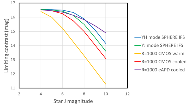
Figure 5. Expected contrast as a function of the target J magnitude for the 2 modes in the SPHERE IFS and for a higher spectral resolution ( R=1000 ) with various assumptions of temperature (warm vs cooled), and read out noise (CMOS vs. eAPD).
