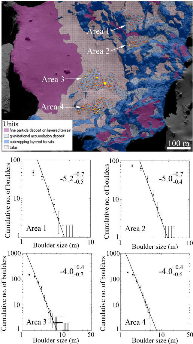
Fig. 10. Power-law indices derived from the cumulative numbers of boulders in four of the largest gravitational accumulation deposits on the Aswan site.
