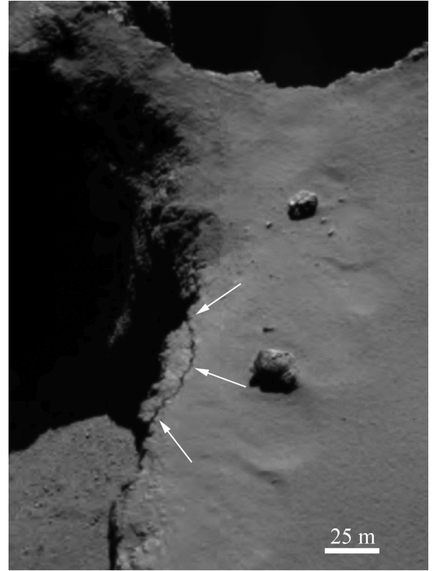
Fig. 11. Fracture of ~50 m located at the edge of the Aswan escarpment. The location of this close-up image is indicated in Fig. 7.
