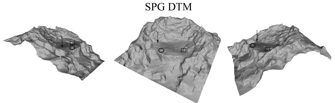
Fig. 4. SPG DTM of the Aswan site with a lateral spacing of 2 m, a true lateral resolution \sim 5\text{--}10 m, and a vertical accuracy \sim 0.1\text{--}0.3 m. The three features identified here correspond to those presented in Fig. 3.
