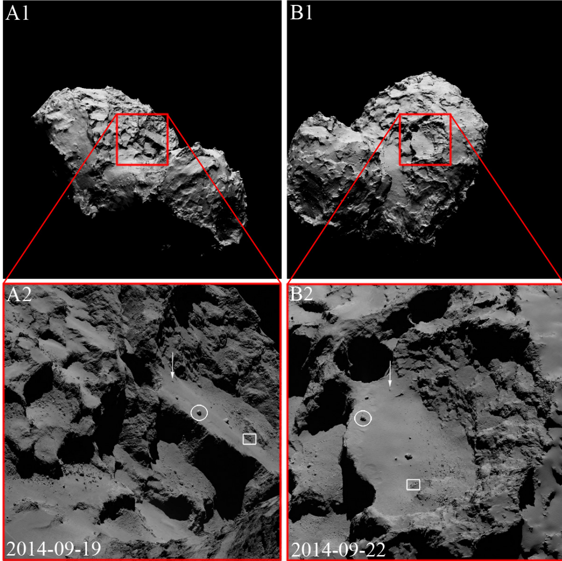
Fig. 3. A1) WAC simulated view of image A2), with the NAC field of view outlined with the red square. A2) NAC image taken on September 19, 2014, showing a side view of the Aswan site. B1) WAC simulated view of image B2) with the NAC field of view outlined with the red square. B2) NAC image taken on September 22, 2014, showing a view from the top of the Aswan site. Three specific features are identified in both images to facilitate understanding the geometry of the observation. The arrow indicates a 5.5 m boulder in close proximity to the 200 m wide pit, the circle shows the boulder (19.3 m wide) closest to the 50 m long fracture presented in Fig. 11, while the rectangle indicates the limit of the outcropping layered terrain.
