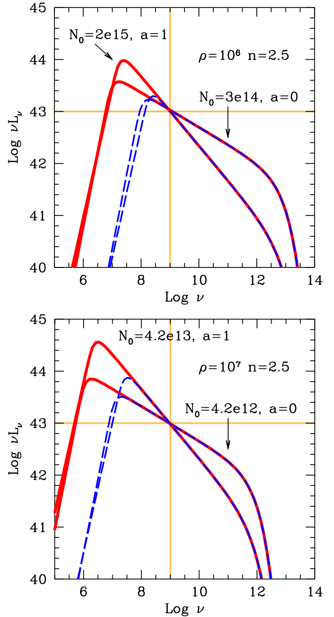
Fig. 3. Spectra, in the \nu - \nu L_\nu representation, produced by a power law distribution of particles accounting for a luminosity of 10^{43} \text{ erg s}^{-1} at 1 GHz. The adopted slope is n = 2.5 . The solid lines show spectra produced by protons; the dashed lines represent the spectra produced by leptons. The different slopes are due to the different a value, controlling the amount of collimation of the radiation, and not to a different slope of the electron distribution. The top panel gives examples for \rho = 10^6 \text{ cm} . The bottom panel shows examples for \rho = 10^7 \text{ cm} . Parameters, listed in Table 1, were found to minimize the required total energy. N_0 indicated in units of \text{cm}^{-3} and \rho in cm.
