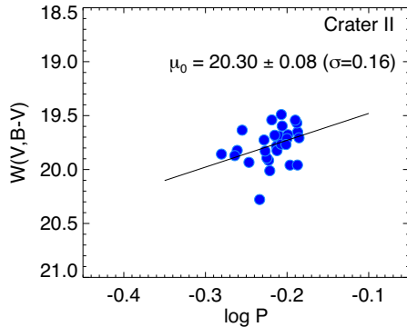
Figure 7. W(V, B - V) - \log P relation for the 24 RRab and the 4 fundamentalized RRs, in Crater II. The black line is the fit of the data to the theoretical slope predicted by Marconi et al. (2015). The zero-point of this relation gives us the first estimation of the distance modulus ( \mu_0 ) for Crater II based on a standard candle.
