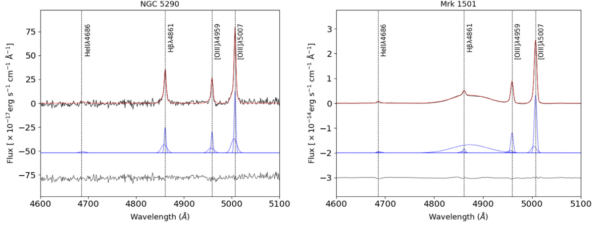
Figure 1. Examples of our fitting method. Left: An example of type 2 AGNs fitting after stellar component subtraction. Right: Spectral fitting of a type 1 AGN after continuum and Fe II subtraction. For each object, we show the spectra (in black), the components fitted for emission lines (in blue), the overall best-fitting model (in red), and the residuals below. The dashed vertical lines mark the location of He II \lambda 4686 , H \beta \lambda 4861 , and [O III] \lambda\lambda 4959, 5007 .
