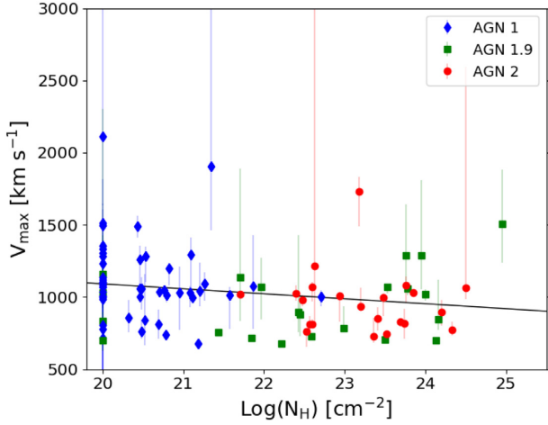
Figure 9. Outflow velocities versus \log(N_H) for the different AGN types.
