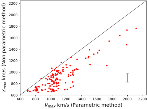
Figure 3. Comparison between maximum outflow velocities estimated using the two detection methods, parametric (x-axis), and non-parametric (y-axis). A typical error bar ( \pm 150 \text{ km s}^{-1} ) is shown for reference.
