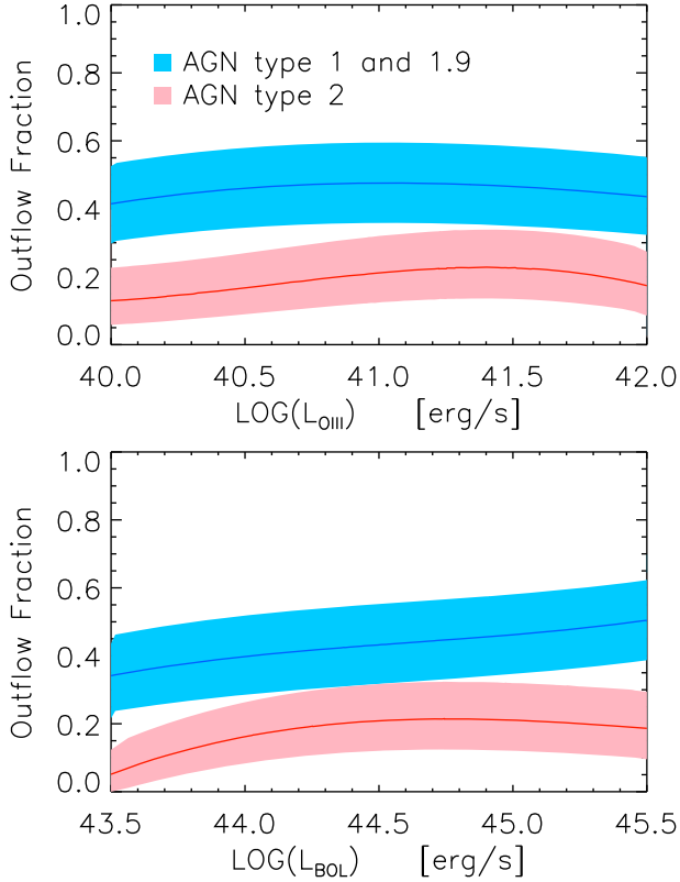
Figure 12. Outflow fraction as a function of luminosities \log L_{\text{O III}} and AGNs \log L_{\text{Bol}} for the different AGN types. Fractions were obtained considering the sample of a fixed number of neighbouring objects in term of luminosity. Then, the resulting curve was then fitted with a low-order polynomial.
