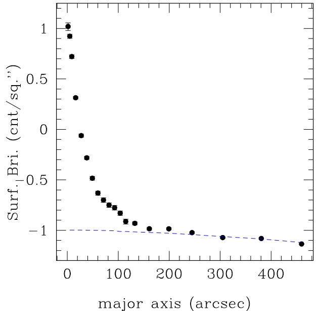
Figure 5. Radial profile of the EPIC-pn data of NGC 1209 in the 0.3–3.0 keV band. The profiles are obtained in concentric elliptical annuli, along the NS/EW direction (left) or azimuthally averaged (right). The dashed lines indicate the profile from the same regions applied to the exposure map and normalized to the data (red/blue for NS/EW, respectively).
