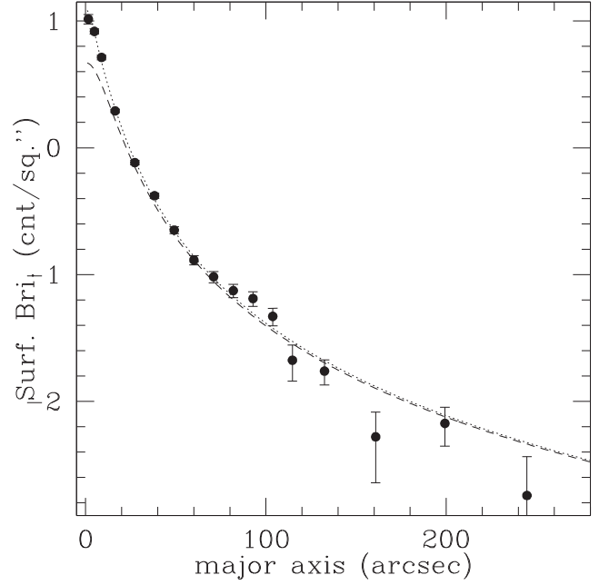
Figure 6. Net radial profile of NGC 1209. The profile can be parametrized (dotted line) by a combination of a \beta -type model, consistent with the point spread function of the EPIC-pn and a second model with \beta = 0.57 and r_0 = 14 \text{ arcsec} (dashed line).
