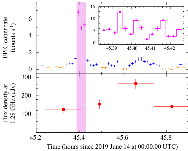
Fig. 3. Zoom of the light curves around the epoch of the brightest X-ray flare ( top ; time bin of 50 s) and the radio flare ( bottom ; time bin of 10 min). The X-ray modes are color-coded as in Fig. 2. The shaded area in magenta marks the epoch of the X-ray flare. The inset in the top panel shows a further zoom of the X-ray light curve at the epoch of the X-ray flare and is binned at 10 s. In all panels, error bars represent 1\sigma uncertainties.
