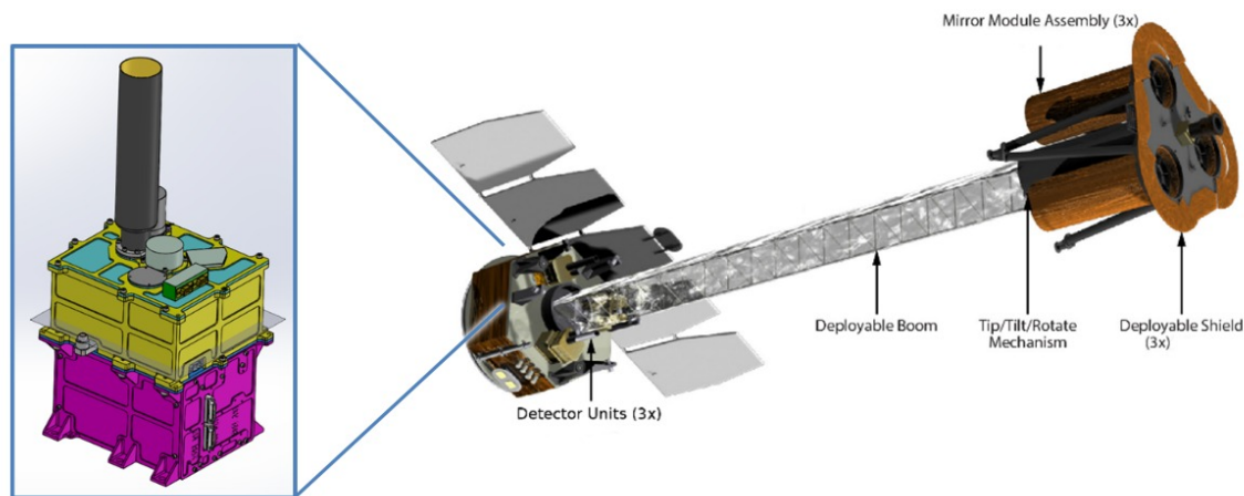
Figure 1. IXPE satellite after on-orbit deployment. A zoom on the DU is on the left.
