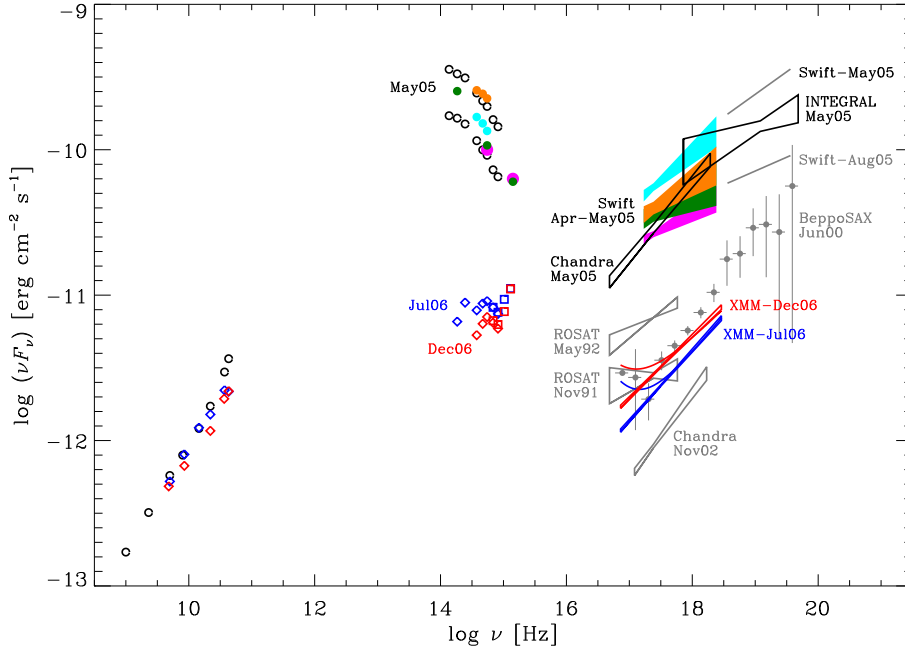
Fig. 7. Broad-band spectral energy distribution of 3C 454.3 (observer's frame). Flux densities derived from the XMM-Newton (EPIC and OM) observations of July and December 2006 are shown in blue and red, respectively. The same colours are used to plot simultaneous low-energy (radio-to-optical) data from observations by the WEBT. The X-ray spectra are displayed as the results of spectral fitting by two models: a power law with Galactic absorption (straight lines) and a double power law with fixed extra absorption (curved lines). X-ray spectra resulting from previous satellite pointings are also shown, in particular those obtained from the Chandra, INTEGRAL, and Swift (XRT and BAT instruments) observations in 2005. Swift-XRT spectra are complemented by simultaneous near-IR-to-UV data from the REM telescope and UVOT detector (Giommi et al., 2006), while radio-to-optical data from the WEBT (open circles) indicate brightness levels during the Chandra and INTEGRAL pointings.
