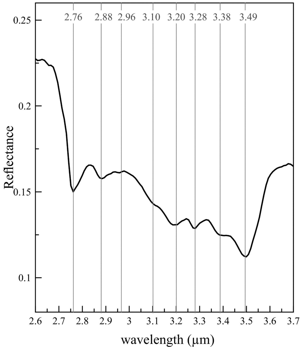
Extended Data Fig. 3 | A typical spectrum of Cerealia facula. An example of spectra of Cerealia facula with highlighted the main features within the 2.6–3.5 micron band.
