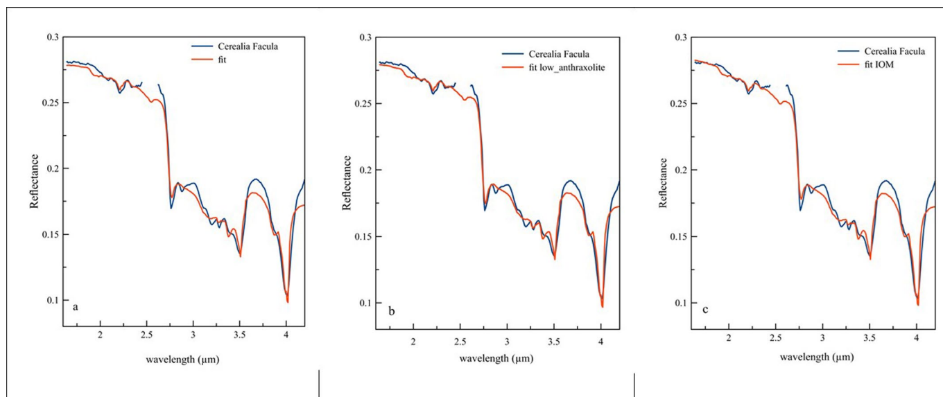
Extended Data Fig. 5 | Spectral fits of the average spectrum of Cerealia facula. The spectrum used for the spectral modelling is an average of the spectra of the pixels on the bright Cerealia facula selected on the basis of the absolute reflectance (median reflectance > 5 times median reflectance of dark surrounding regions, in the range 2.6 – 3.4 μm). Dataset used is described in Extended Data Table 4. A) spectral fit using the species reported in Extended Data Table 3, without organics; B) spectral fit using the species reported in Extended Data Table 3, including low-anthraxolite; C) spectral fit using the species reported in Extended Data Table 3, including IOM. The data 2.5 micron has been removed because affected by the detector filters.
