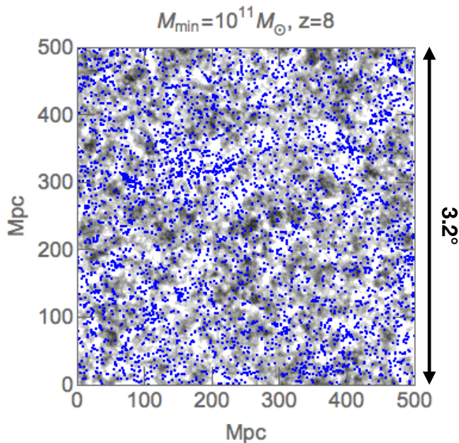
Figure 7. Distribution of dark halos with M_h \geq 10^{11} M_\odot at z = 8 (blue dots) superimposed on the background ionization field (grey scale) taken from the simulated tomographic map at z = 8 shown over an area of 500 Mpc (comoving) on a side, which corresponds to 3.2^\circ . This map was smoothed over a scale of 30 Mpc. The darker (brighter) regions correspond to more neutral (ionized) regions. Both distributions were projected from a 100-Mpc thick slice at z = 8 . The map of ionization field was produced based on the FULL model of Sobacchi & Mesinger (2014).
