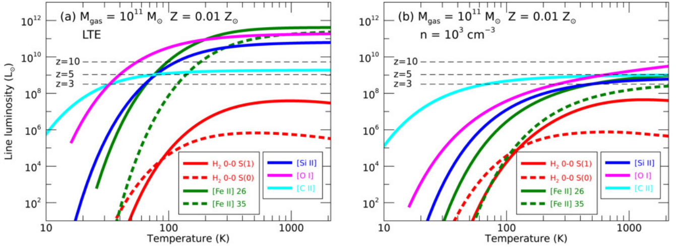
Figure 5. Luminosities of \text{H}_2 lines (0–0 S(1) 17\,\mu\text{m} and 0–0 S(0) 28\,\mu\text{m} ) and fine-structure lines ([Fe II] 25.99/35.35\,\mu\text{m} , [Si II] 34.8\,\mu\text{m} , [O I] 63\,\mu\text{m} , and [C II] 158\,\mu\text{m} ) calculated for a low-metallicity ( Z = 0.01\,M_\odot ) forming galaxy with a gas mass of 10^{11}\,M_\odot . The left panel (a) assumes a gas density high enough for these lines to be thermalized (i.e., in LTE) while the right panel (b) corresponds to the case with a gas density of 10^3\,\text{cm}^{-3} . A molecular fraction of 2 \times 10^{-4} was assumed for both cases. The former is similar to the calculation presented by Santoro & Shull (2006) (see their Figure 11 for a similar model with a gas mass of 10^8\,M_\odot ). The horizontal dotted lines indicate the nominal 5\sigma detection limit of SAFARI with a 10-hour on-source integration time for z = 3, 5 , and 10 . The LTE case on the left suggests that if the gas is sufficiently warm ( T \gtrsim 200\,\text{K} ), fine-structure lines like [Fe II] 25.99/35.35\,\mu\text{m} and [Si II] 34.8\,\mu\text{m} can be quite luminous (note, however, that these lines will be redshifted out of the SAFARI window at z = 7.8/5.5 , and 5.6 , respectively).
