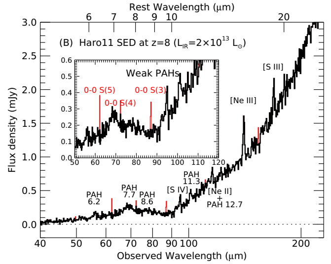
Figure 3. SAFARI 10-hr LR ( R=300 ) spectra for z=8 galaxies simulated for the following three-types of galaxies: (A) HLSJ0918, a HyLIRG at z=5.24 (see Figure 1 and Table 1); (B) Haro 11, a low-metallicity infrared-luminous local BCD; and (C) II Zw 40, another low-metallicity local BCD that is not infrared-luminous. For HLSJ0918, the L_{\text{IR}} = 10^{11.75} L_{\odot} LIRG SED from Rieke et al. (2009) was used as in Figure 1, while for the two BCDs, the fully-processed Spitzer /IRS low-resolution spectra were obtained from the Combined Atlas of Sources with Spitzer IRS Spectra (CASSIS; Lebouteiller et al. 2011). The infrared luminosities of these SEDs have been scaled to 2 \times 10^{13} L_{\odot} , comparable to the intrinsic luminosity of HFLS3. See the caption of Figure 1 for how these SAFARI spectra were simulated. The red lines show simulated \text{H}_2 emission lines (assumed to be unresolved) produced by 2 \times 10^{10} M_{\odot} of T=200 K gas and 2 \times 10^8 M_{\odot} of T=1000 K gas under the LTE assumption (an ortho-to-para ratio of 3:1 is also assumed). These \text{H}_2 lines are hardly visible in the original galaxy spectra.
