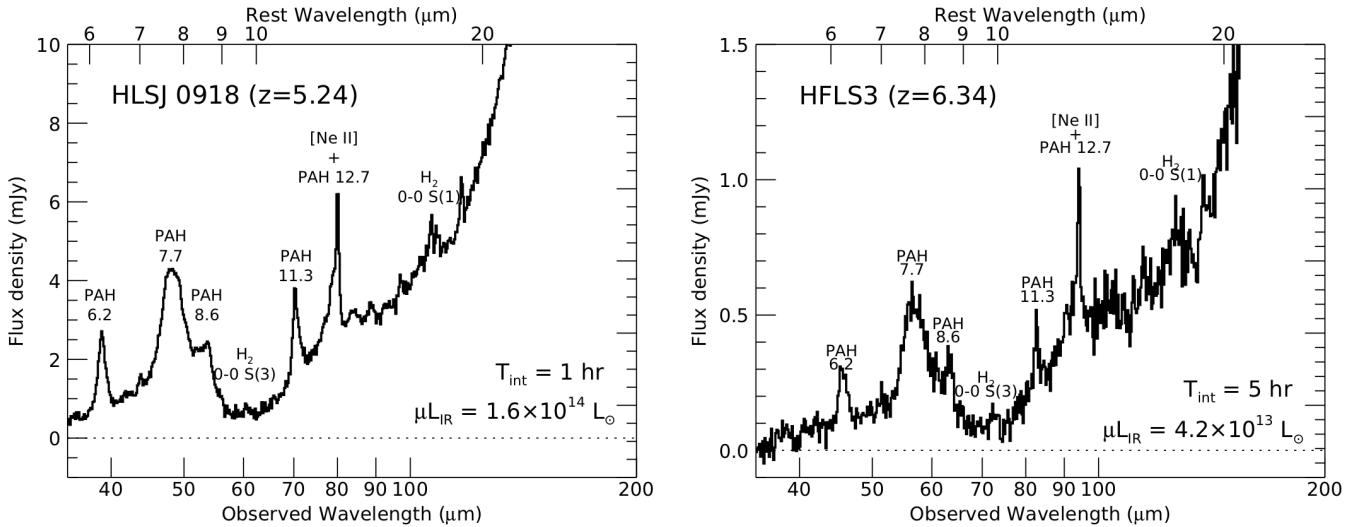
Figure 1. Simulated SAFARI spectra of HLSJ0918 ( z = 5.24 , \mu = 9 : Combes et al. 2012; Rawle et al. 2014) and HFLS3 ( z = 6.34 , \mu = 2 : Riechers et al. 2013; Cooray et al. 2014) are shown in the left and right panels, respectively. The average local galaxy SED templates (Rieke et al. 2009) of L_{\text{IR}} = 10^{11.75} and 10^{12.50} L_{\odot} were used, respectively, which produce good fits to the observed rest-frame far-infrared SEDs of these galaxies. The template SEDs were first scaled to the infrared luminosities without a lensing correction ( \mu L_{\text{IR}} in each panel) and then fit with PAHFIT (Smith et al. 2007) with a pixel sampling of R = 600 . These PAHFIT-produced model spectra were then redshifted and noise-added for corresponding integration times ( T_{\text{int}} in each panel). Finally, the resultant spectra were resampled with R = 300 pixels. However, the effective resolution of these simulated spectra is less than R = 300 due to the low resolution ( R \approx 60\text{--}130 ) of the Spitzer /IRS data used by Rieke et al. (2009) to build templates. Note that the actual mid-infrared spectra of these z > 5 galaxies may significantly differ from those of local LIRGs/ULIRGs (see Section 2.4 for more discussion).
