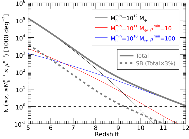
Figure 6. Cumulative surface densities of DM halos per 1000 \text{deg}^2 as predicted by the the standard \Lambda\text{CDM} model. The black line indicates the cumulative surface density of \geq 10^{12} M_\odot halos down to given redshifts while the blue and red lines plot the corresponding numbers for \geq 10^{11} M_\odot halos gravitationally lensed by a factor of \geq 10\times ( \mu \geq 10 ) and for \geq 10^{10} M_\odot halos lensed by a factor of \geq 100\times ( \mu \geq 100 ), respectively. According to the calculation by Zackrisson et al. (2015), when the source redshift is above \sim 5 , the corresponding lensing probability is roughly constant and \sim 10^{-4} for \mu \geq 10 and \sim 10^{-6} for \mu \geq 100 along an average line of sight. These probabilities have been multiplied with the \geq 10^{11} and \geq 10^{10} M_\odot halo surface densities. The thick grey line plots the total surface density of the three halo populations combined while the thick grey dashed line plots 3% of the total number, comparable to the starburst fraction estimated at lower redshift (e.g., Béthermin et al. 2017). The halo comoving number density was computed with the Press-Schechter formalism (Press & Schechter 1974). The horizontal dashed line corresponds to N = 1 .
