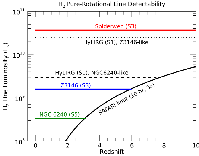
Figure 4. Detectability of \text{H}_2 pure-rotational lines for three known extreme \text{H}_2 emitters: (1) the Spiderweb radio galaxy at z = 2.16 with L(0-0 \text{ S}(3)) = 3.7 \times 10^{10} L_{\odot} (Ogle et al. 2012); (2) Z3146 BCG at z = 0.29 with L(0-0 \text{ S}(3)) = 1.6 \times 10^9 L_{\odot} (Egami et al. 2006a); (3) NGC 6240 at z = 0.0245 with L(0-0 \text{ S}(3)) = 3.4 \times 10^8 L_{\odot} (Armus et al. 2006). The brightest line was used for each case. With SAFARI’s line sensitivity, which is also plotted (10 hours, 5\sigma ), the Spiderweb galaxy would be visible beyond z = 10 , while the Z3146 BCG would be visible up to z \sim 6 ; NGC 6240, on the other hand, would drop out at z \sim 3 . Also shown are the visibilities of a HyLIRG ( L_{\text{IR}} = 10^{13} L_{\odot} ) through the 0–0 S(1) line assuming L_{0-0 \text{ S}(1)}/L_{\text{IR}} = 0.25\% (Z3146-like) and 0.03% (NGC 6240-like).
