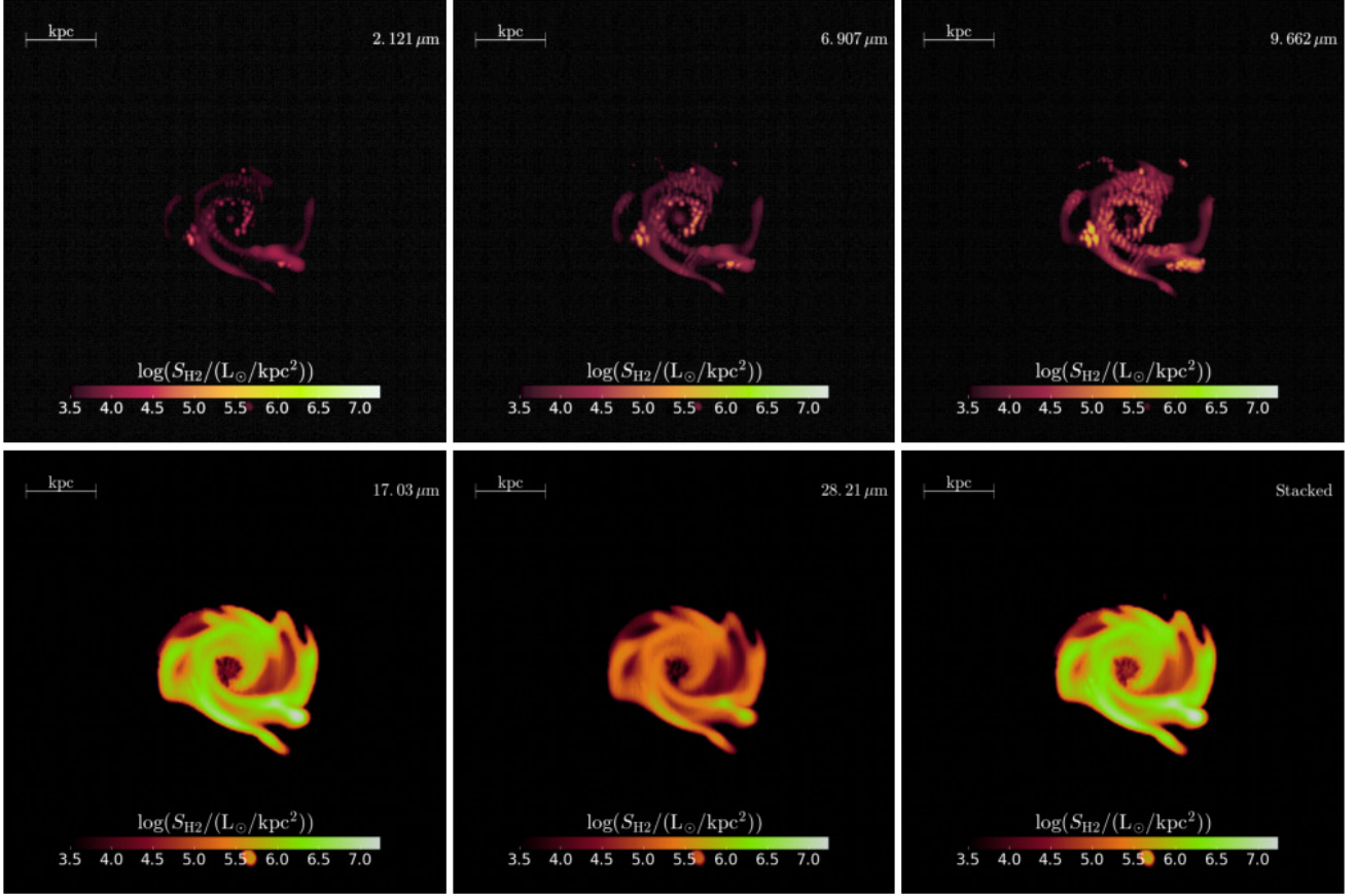
Figure 8. Synthetic \text{H}_2 line emission for the z=6 galaxy Althaea (Pallottini et al. 2017b). The lines shown are (from top left to bottom right) 1-0 S(1) 2.12\ \mu\text{m} , 0-0 S(5) 6.91\ \mu\text{m} , 0-0 S(3) 9.66\ \mu\text{m} , 0-0 S(1) 17.0\ \mu\text{m} , and 0-0 S(0) 28.2\ \mu\text{m} . The last panel at bottom right shows the stacked sum of all the lines, which is dominated by the 0-0 S(1) line.
