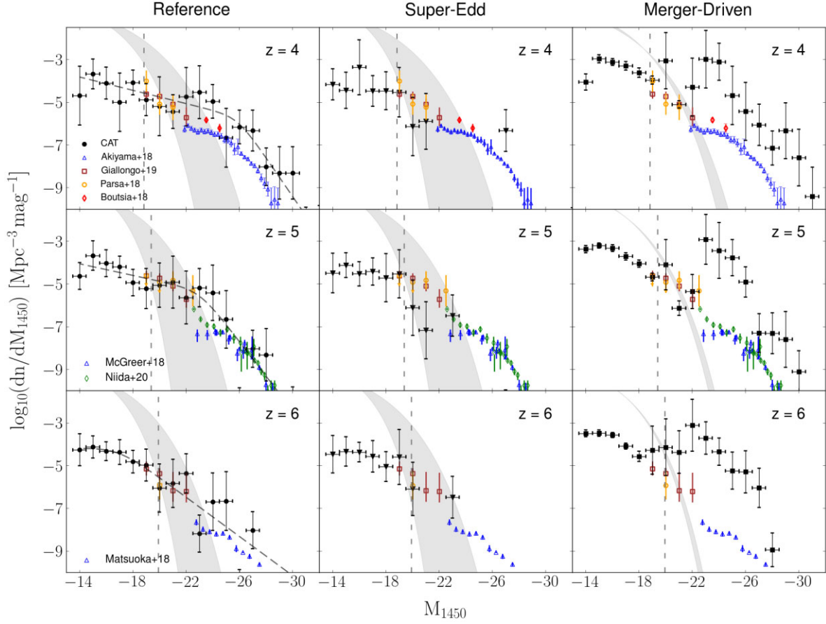
Figure 9. The AGN UV LFs at z = 4, 5 , and 6 (from top to bottom). Each column shows the results obtained in one of the three CAT models: the reference model (left-hand panels), the super-Edd model (central panels), and the merger-driven model (right-hand panels). The black data points represent the predicted AGN LFs, properly corrected for obscuration as described in the text. The black dashed line shows the best fit for the Reference model. The grey shaded area encloses the region between the intrinsic and the dust-corrected galaxy UV luminosity function predicted by each model at the corresponding redshift. The coloured data represent the observational constraints on the AGN LF obtained by Parsa, Dunlop & McLure (2018, orange circles), Boutsia et al. (2018, red diamonds), Giallongo et al. (2019, brown squares), by the SHELLQs survey (Matsuoka et al. 2018), the CFHT Legacy Survey (McGreer et al. 2018), and the Hyper Suprime-Cam Wide Survey (Akiyama et al. 2018; Niida et al. 2020) (blue triangles and green diamonds). The vertical black dashed lines show the JWST luminosity limit at each redshift predicted by Griffin et al. (2020).
