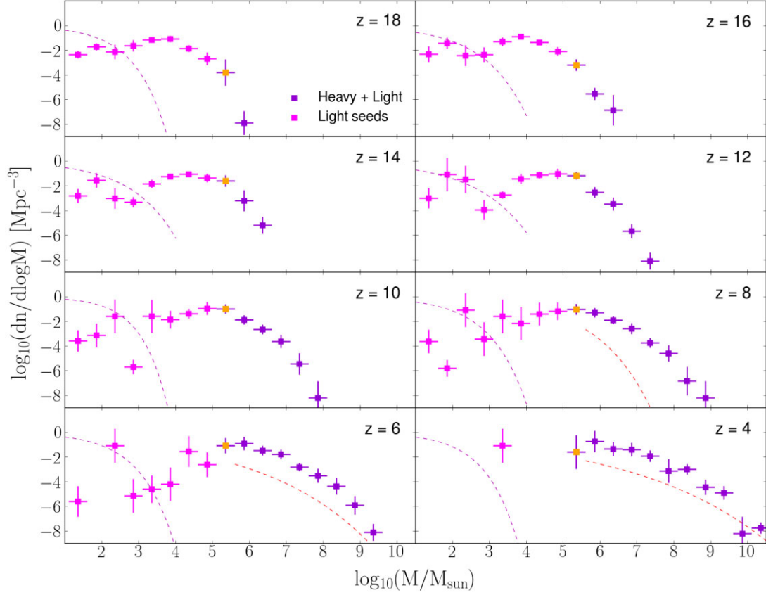
Figure 6. Same as Fig. 5 but for the merger-driven accretion model (see Section 2.4.2). Here, we show with violet data points the mass bins above 10^5 M_\odot since, unlike the previous models, they are now populated by both light and heavy BH seed descendants. Distributions (data points with error bars) are compared with best fits obtained for the reference model (dashed lines).
