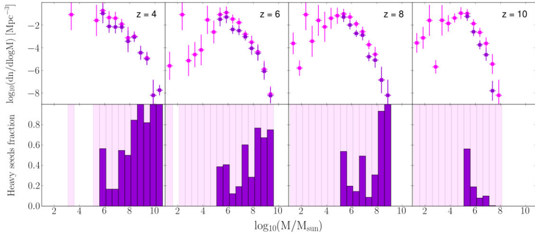
Figure 7. The figure shows, for the merger-driven model, the relative contribution to the final BH MF of BHs descending from at least one heavy or only light BH seeds. Top row: the total BH MF (magenta points, same as in Fig. 6) and the contribution of only heavy -BH seeds descendants (violet) at z = 4, 6, 8 , and 10 (from left to right). Bottom row: the corresponding percentage of heavy BH seed descendants in different mass bins. BHs descending only from light -BH seeds (represented by lighter magenta regions of the histograms) clearly provide, in this model, a significant contribution to the global MF, even at the high-mass end.
