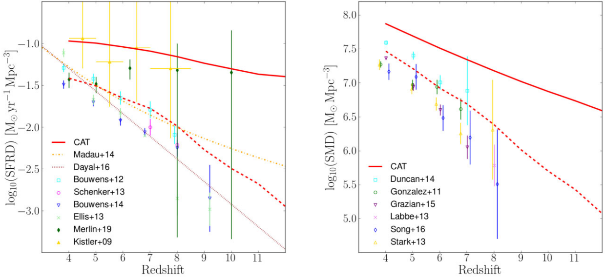
Figure 2. Redshift evolution of the comoving SFRD (left-hand panel) and stellar mass density (right-hand panel) predicted by CAT, when the entire galaxy population is considered (red solid lines) and when only galaxies with M_{UV} < -17.7 are accounted for (red dashed lines). In each panel, the model predictions are compared with different observational results, as indicated in the legends Kistler et al. (2009), González et al. (2011), Bouwens et al. (2012), Labbé et al. (2013), Stark et al. (2013), Schenker et al. (2013), Ellis et al. (2013), Duncan et al. (2014), Bouwens et al. (2014), Oesch et al. (2014), Grazian et al. (2015), Song et al. (2016), and Merlin et al. (2019). In the right-hand panel, the yellow dash-dotted line shows the empirical SFRD by Madau & Dickinson (2014) and the brown dotted line shows the model prediction by Dayal, Ward & Cockell (2016).
