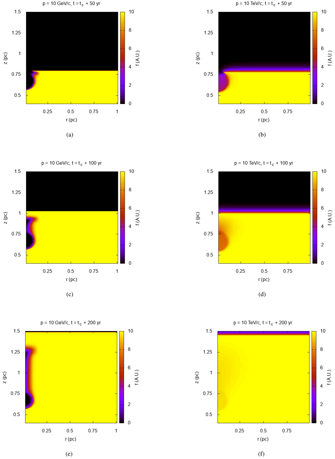
Figure 6. Distribution function of CR protons of momentum (a,c,e) 10 GeV/c and (b,d,f) 10 TeV/c at different times with respect to t_c : panel (a) and (b) are at t = t_c + 50 yr, (c) and (d) are at t = t_c + 100 yr, while (e) and (f) are at t = t_c + 200 yr. The precursor presence in front of the shock is well visible at 10 TeV.
