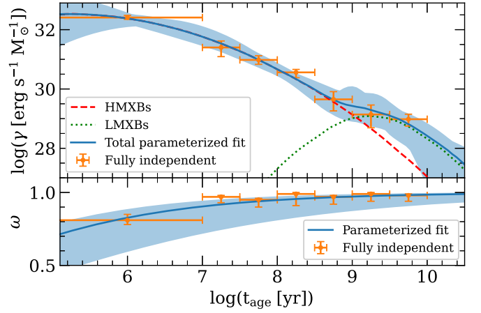
Figure 11. The parameterized fits for \gamma and \omega presented alongside the results from the fully independent model (orange points). Top: the parameterized formula for \gamma can be decomposed into the contributions from HMXBs and LMXBs (shown as the red dashed and green dotted lines, respectively). The constraints become very weak above 9.75 Gyr because that is the assumed age of the oldest age bin in this study. The shaded region shows the uncertainty as derived from the top 68% of the fully independent model results (“top” is defined by having the lowest C value). Bottom: the parameterized fit of \omega is shown with a similar uncertainty region reflecting the top 68% of results.
