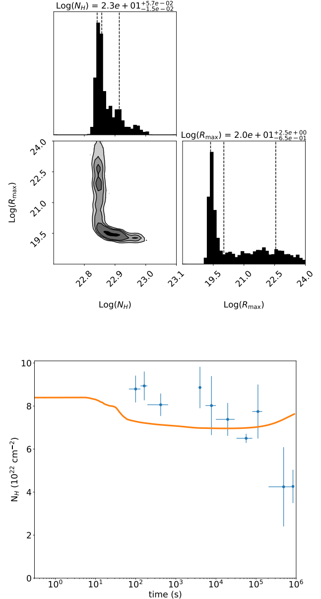
Fig. 3. Results of the photoionization code fit of the column density evolution with time. Top : results from the MCMC simulation for modeling via time-dependent photo-absorption. Bottom : corresponding best fit model from photo-absorption. The large \chi^2_{\text{red}} \sim 5 shows that time-dependent absorption is not a good explanation for the observed time-variable absorption.
