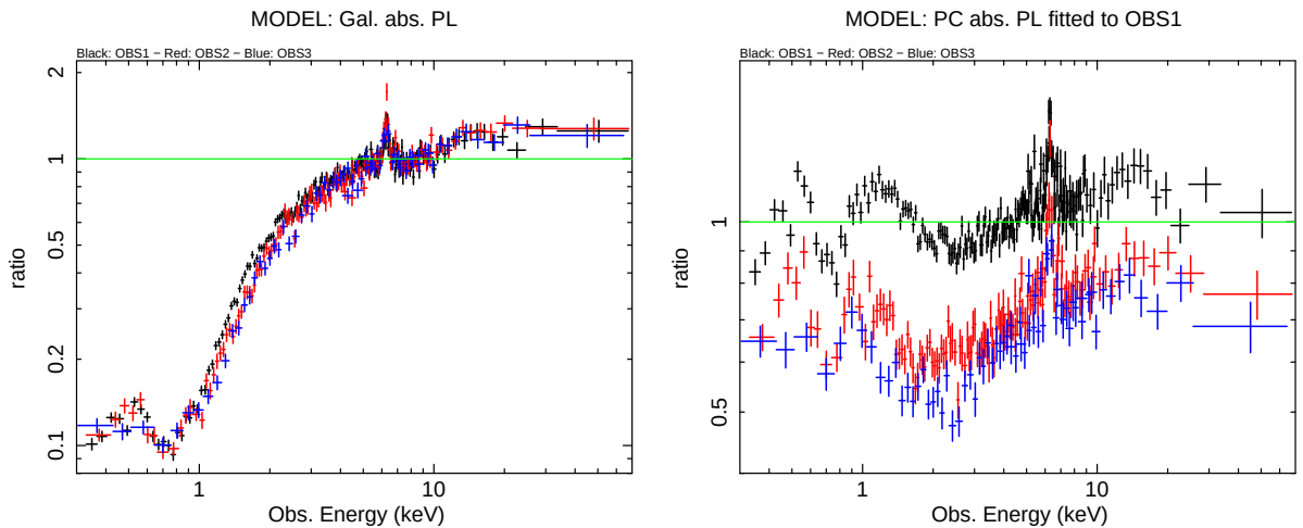
Figure 4. Data-to-model ratio for the XMM-Newton pn and NuSTAR FPMA spectra: black, OBS 1; red, OBS 2; blue, OBS 3. All data are rebinned for clarity. Left: the model is a power law, fitted to the data between 5 and 10 keV ( \Gamma \sim 1.53 ), absorbed by our Galaxy. Right: a partial covering neutral absorber is added to the model and fitted to the OBS 1 data considering the whole energy range.
