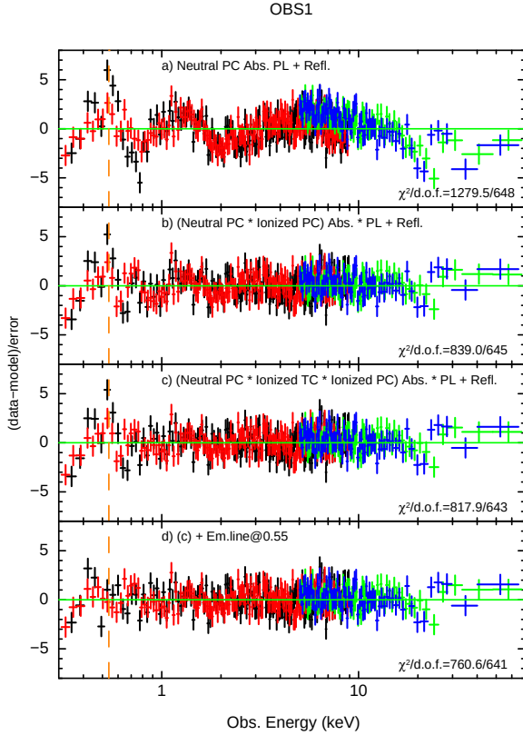
Figure 5. Relevant residuals, plotted in terms of sigmas with error bars of size one, when different models are applied to the XMM-Newton (black, pn; red, MOS) and NuSTAR (green, FPMA; blue, FPMB) spectra of Mrk 915 as recorded during the OBS1 observation: from top to bottom, a continuum composed by the intrinsic power law and a reflection component is view through a partially covering neutral absorber (panel a); in panel b) we present the residuals when a partially covering ionized absorber is included, while in panel c) a second ionized layer has been added. Finally, panel d) shows the residuals when the model includes also the soft X-ray emission line; its position is marked in all panels with a vertical orange dashed line. All data are rebinned for clarity.
