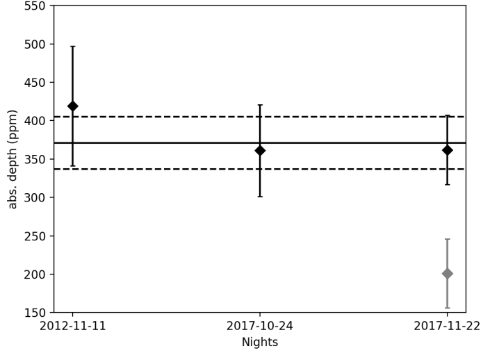
Fig. 7. The absorption depth of the three nights calculated from the transmission spectrum of the sodium doublet plotted with the value for all nights together highlighted as a black horizontal line. The dashed lines mark one sigma around the main absorption depth. The data point in gray shows the value calculated for Night 3 when the cloud contaminated exposures are not discarded. All values were taken from Tables 7 and 6.
