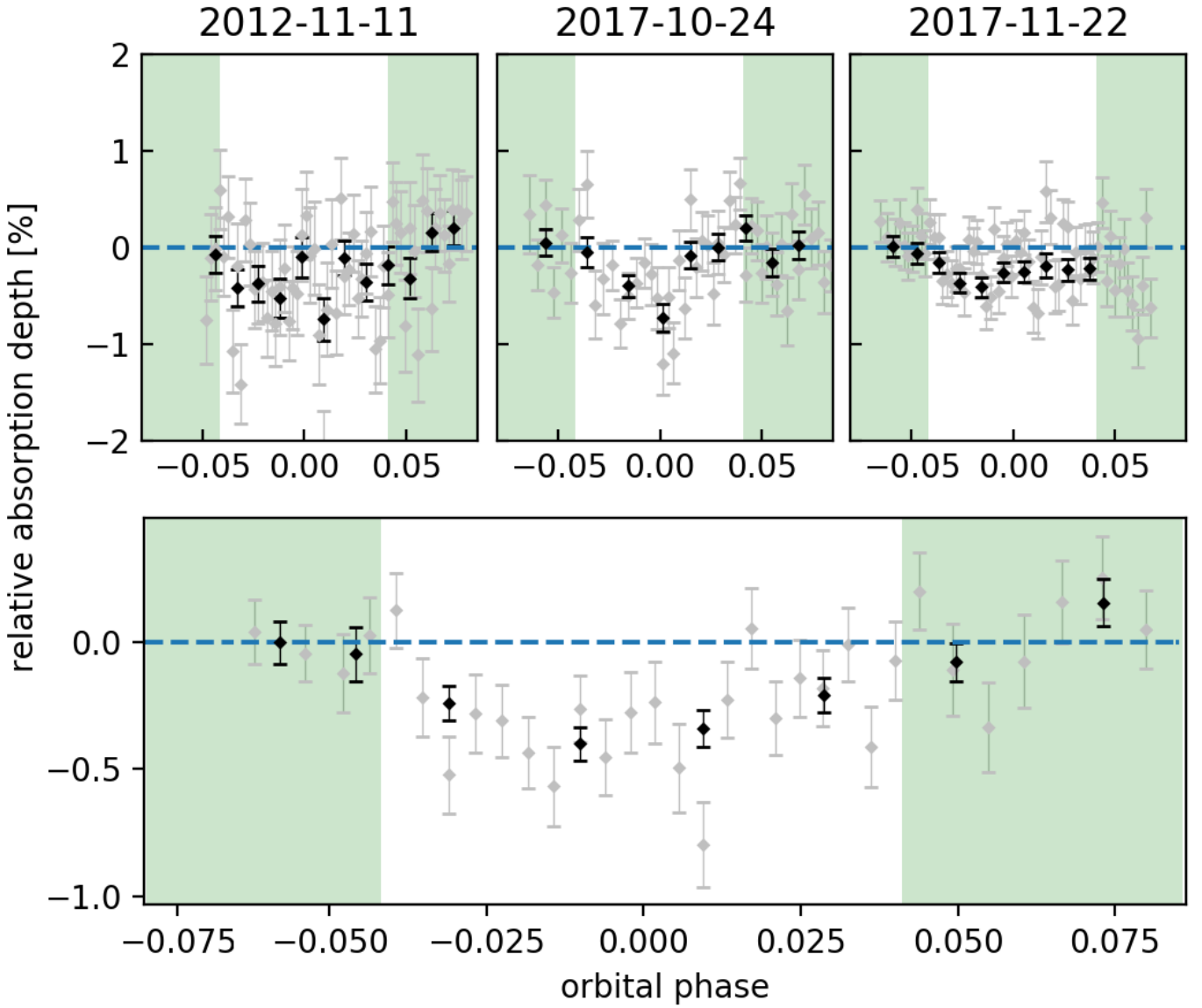
Fig. 5. HARPS relative excess absorption in the sodium doublet compared to the white light curve of WASP-76b evolving in time. The upper three plots show the light curves for each night 2012-11-11, 2017-10-24 and 2017-11-22 from left to right. Note the different scales on the ordinate axis for the upper and lower panel and the influence of stratus-clouds in the out-of-transit exposures during the night of 2017-11-22. The grey data points show the relative absorption for each exposure, in black the data is binned by 5 spectra. The lower panel shows the light curve for all three nights combined, with the exposures averaged together with bins of 5 spectra in grey. The green background marks the exposures taken out-of-transit.
