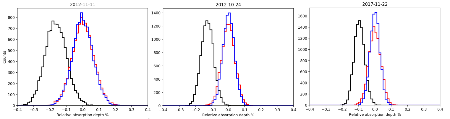
Fig. 8. Distributions of the empirical Monte-Carlo analysis for the 12 Å passband. The results for the transmission spectrum method are shown. As expected the 'in-in' (red) and 'out-out' (blue) distributions are centred around 0 (no planetary detection) and the randomised 'in-out' distribution shows a detection (black). In each night a different number of spectra was taken, which means that each randomisation will give a different number of counts, which results in a different scaling on the y-axis. This has no influence on the overall result.
