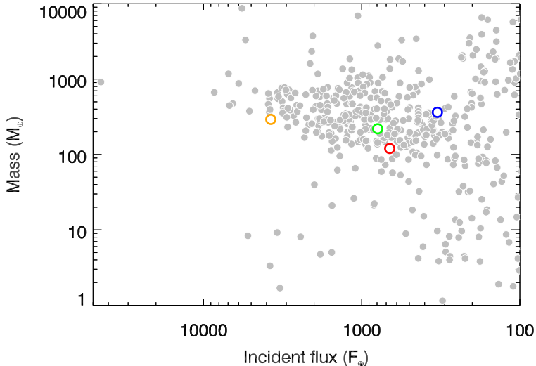
Fig. 1. Mass of the planet vs. bolometric optical and infrared incident flux in units of flux received at Earth. In grey, transiting exoplanets are shown with V < 16 and masses determined with a precision better than 20 %. WASP-76b is shown in orange. For comparison WASP-49b (Wyttenbach et al. 2017), HD 189733b (Wyttenbach et al. 2015) and HD 209458b (for reference) are shown in red, blue and green respectively.
